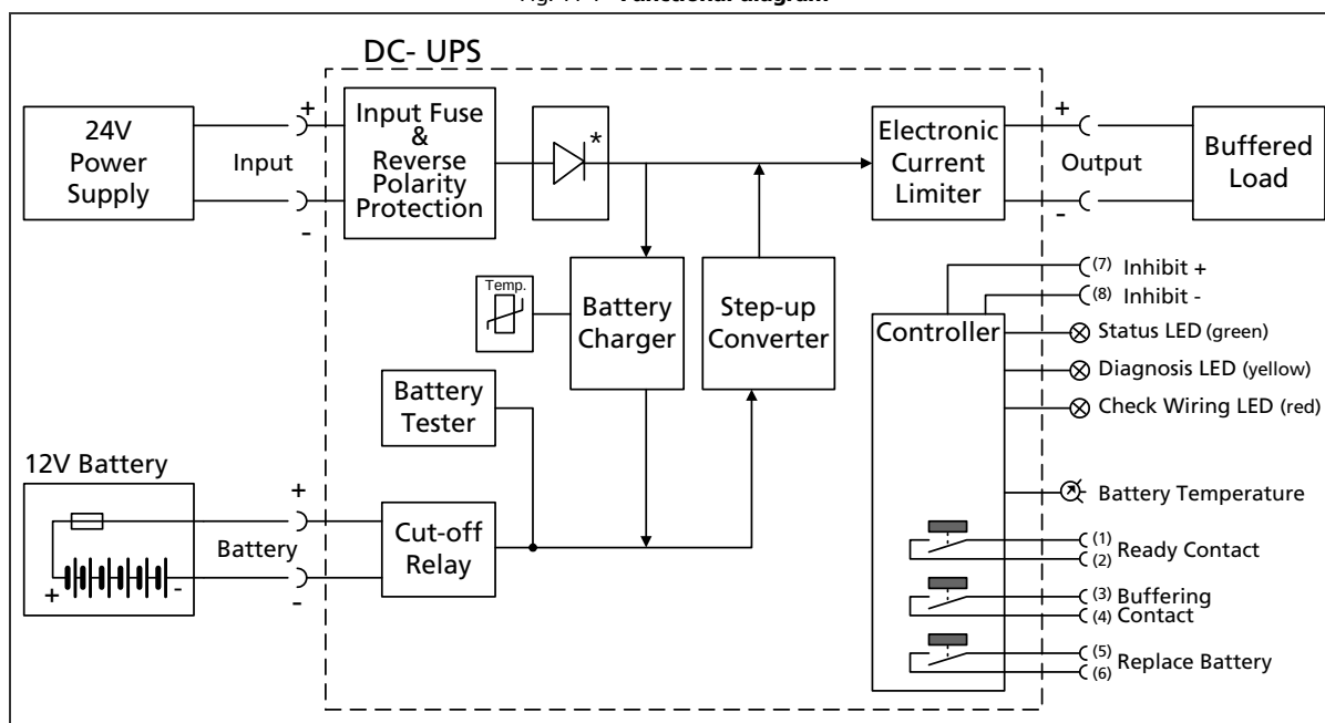
Fig. 11-1 Functional diagram
