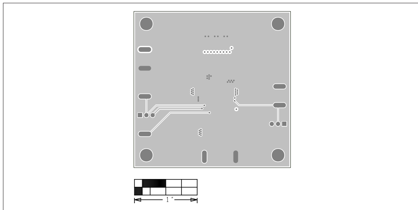
MAX17536 3.3V Output EV Kit PCB Layout—Layer 2 Ground
