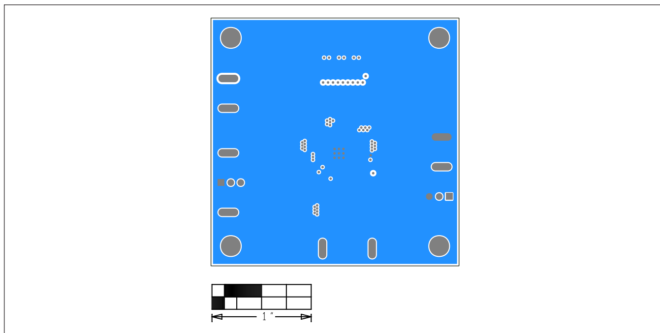
MAX17536 3.3V Output EV Kit PCB Layout—Bottom Layer
