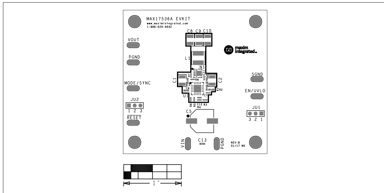
MAX17536 3.3V Output EV Kit PCB Layout—Silk Top
