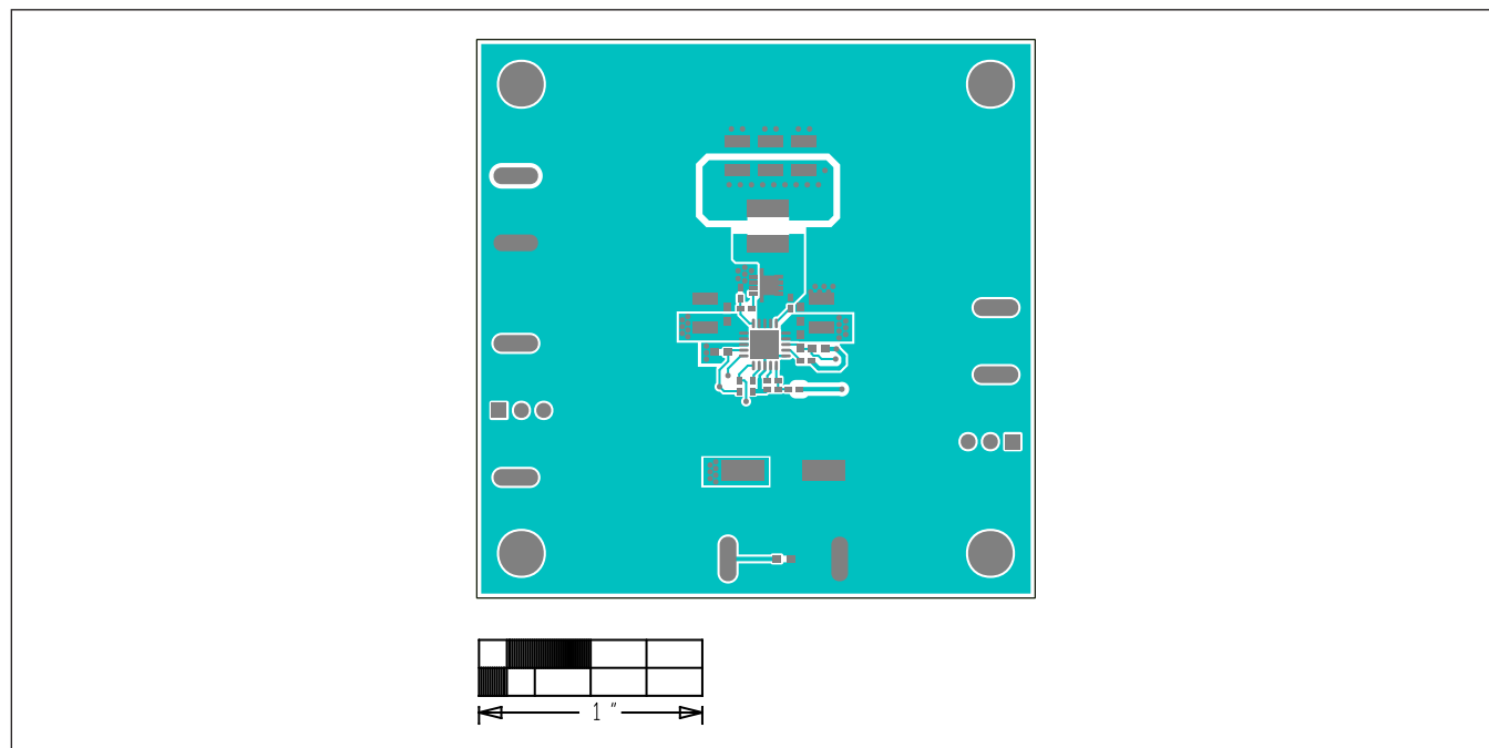
MAX17536 3.3V Output EV Kit PCB Layout—Top Layer
