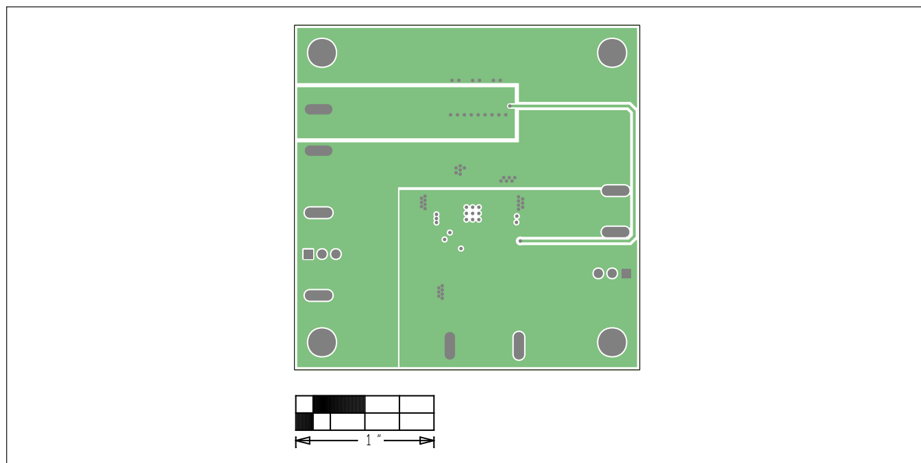
MAX17536 3.3V Output EV Kit PCB Layout—Layer 3 Power
