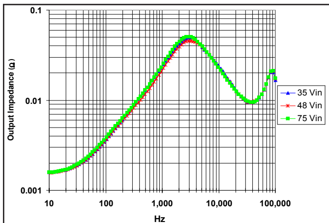
Figure 25: Output impedance ( Z_{out1} = V_{out1}/I_{out1} ) for minimum, nominal, and maximum input voltage at full rated power, for 1.5V output.
