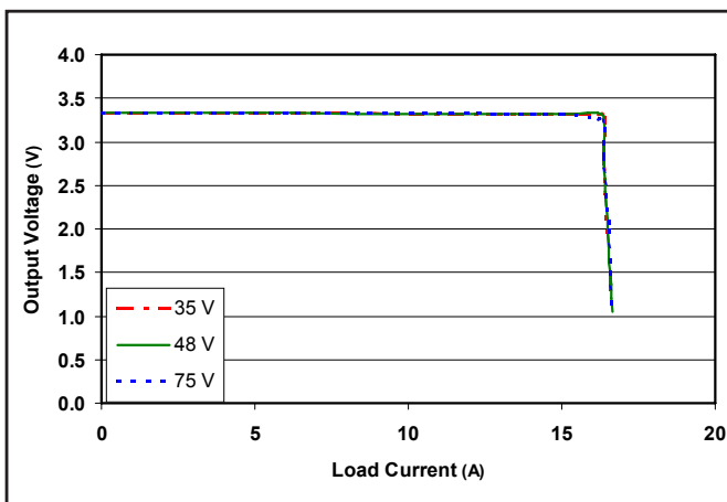
Figure 22: Output voltage vs. load current showing typical current limit curves and converter shutdown points for the 3.3V output. 1.5V load is at 0A.
