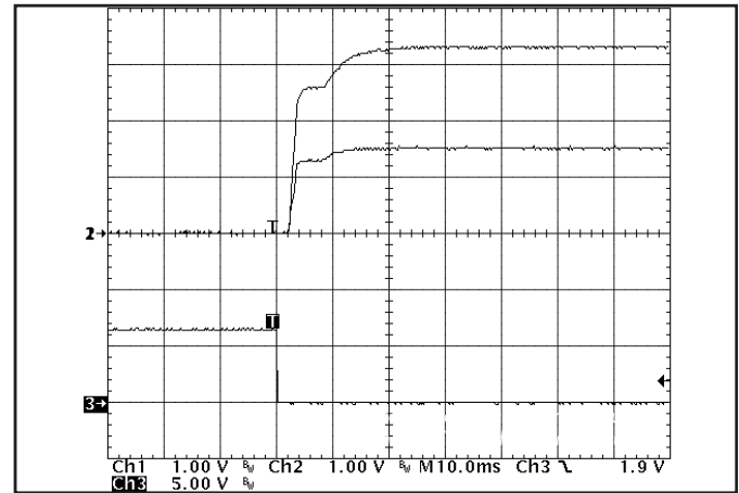
Figure 14: Turn-on transient at zero load current (10 ms/div). Ch 1: 1.5Vout (1V/div); Ch 2: 3.3Vout (1V/div) Ch 3: ON/OFF input (5V/div)
