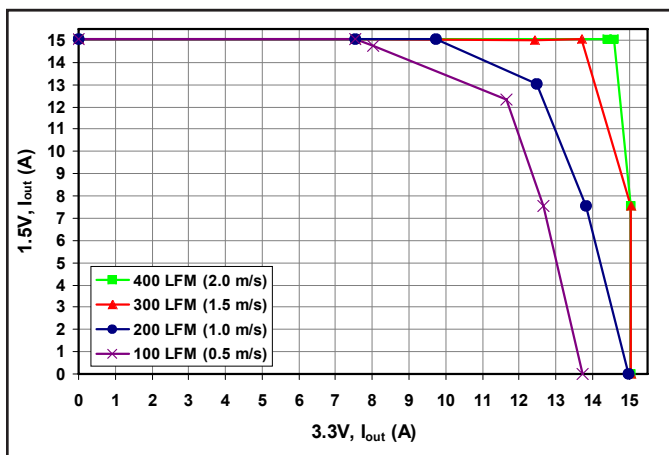
Figure 9: Maximum output power derating curves at 70°C vs. airflow rates of 100 through 400 LFM. Curve shows available current for 1.5V rail on y axis and available current for 3.3V rail on x axis. (nom. Vin)
