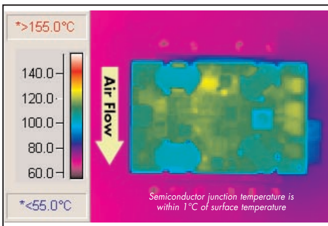
Figure 10: Thermal plot of converter at 13A load on 1.5V output and 12.5A load on 3.3V output with 70°C air flowing at 200 LFM. Air flow across the converter is from pin 1 to pin 3 (nominal input voltage).
