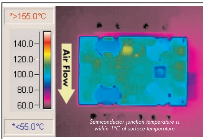
Figure 8: Thermal plot of converter at 15A load on 1.5V output and 14A load on 3.3V output with 55°C air flowing at 200 LFM. Air flow across the converter is from pin 1 to pin 3 (nominal input voltage).
