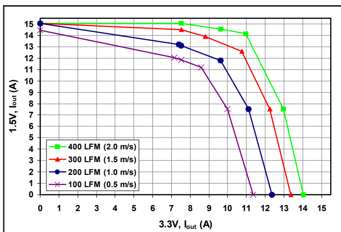
Figure 11: Maximum output power derating curves at 85°C vs. airflow rates of 100 through 400 LFM. Curve shows available current for 1.5V rail on y axis and available current for 3.3V rail on x axis. (nom. Vin)
