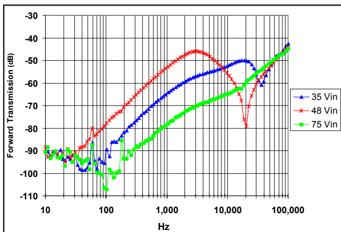
Figure 27: Forward Transmission ( FT_1 = V_{out1}/V_{in} ) for minimum, nominal, and maximum input voltage at full rated power, for 1.5V output.
