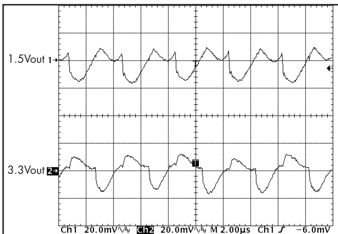
Figure 20: Output Voltage Ripple at nominal input voltage and rated load current on both outputs (20 mV/div). Load capacitance: 1 \mu F ceramic & 15 \mu F tantalum. Bandwidth: 20 MHz. (see Fig. 17)
