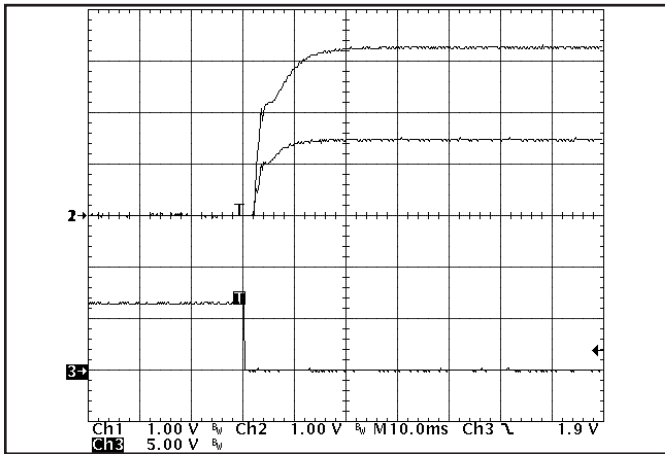
Figure 13: Turn-on transient at full rated load current (resistive load) (10 ms/div). Ch 1: 1.5Vout (1V/div); Ch 2: 3.3Vout (1V/div) Ch 3: ON/OFF input (5V/div)
