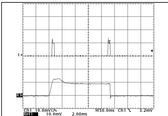
Figure 24: Load current for 3.3V output (20A/div) as a function of time when the converter attempts to turn on into a 10 m \Omega short circuit. Bottom trace is an expansion of the on-time portion of the top trace.
