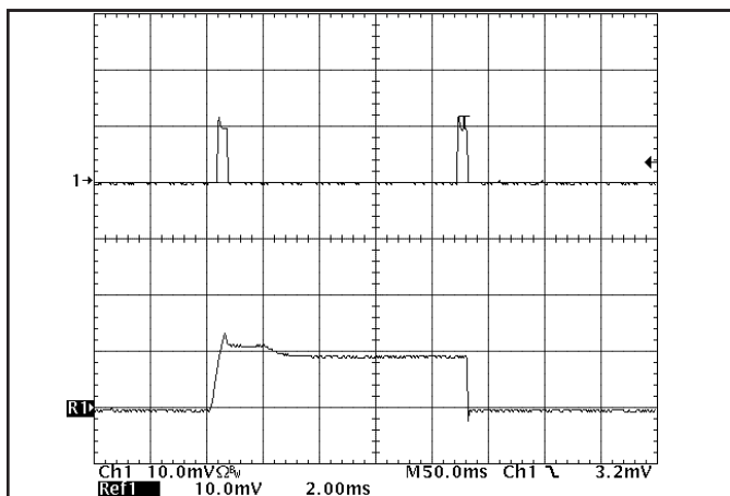
Figure 23: Load current for 1.5V output (20A/div) as a function of time when the converter attempts to turn on into a 10 m \Omega short circuit. Bottom trace is an expansion of the on-time portion of the top trace.
