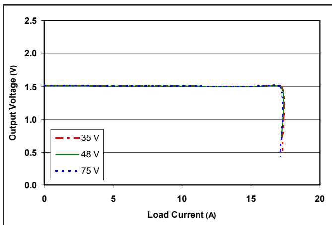
Figure 21: Output voltage vs. load current showing typical current limit curves and converter shutdown points for the 1.5V output. 3.3V load is at 0A.
