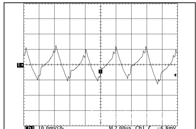
Figure 18: Input Terminal Ripple Current, 1.5V & 3.3V outputs at full rated output current and nominal input voltage with 10μH source impedance and 100μF electrolytic capacitor (10 mA/div). (see Fig. 17)
