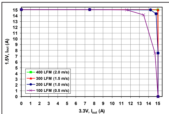
Figure 7: Maximum output power derating curves at 55°C vs. airflow rates of 100 through 400 LFM. Curve shows available current for 1.5V rail on y axis and available current for 3.3V rail on x axis. (nom. Vin)
