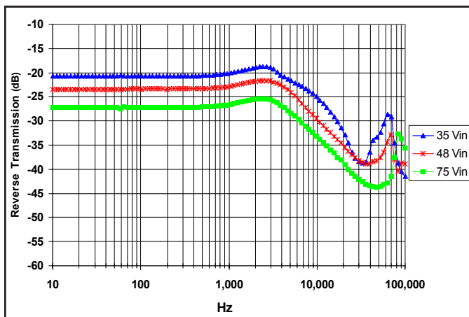
Figure 29: Reverse Transmission ( RT_1 = I_{in}/I_{out1} ) for minimum, nominal, and maximum input voltage at full rated power, for 1.5V output.
