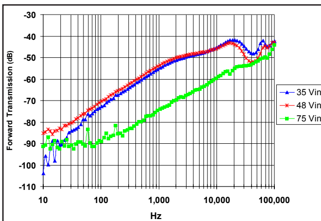
Figure 28: Forward Transmission ( FT_2 = V_{out2}/V_{in} ) for minimum, nominal, and maximum input voltage at full rated power, for 3.3V output.
