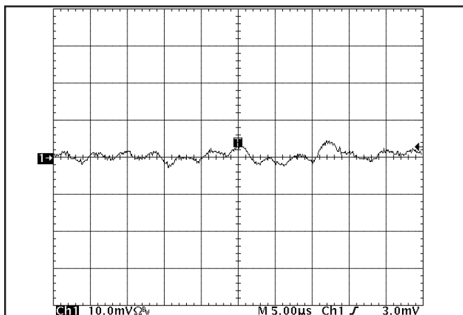
Figure 19: Input Reflected Ripple Current, i_s , through a 10 \mu H source inductor at nominal input voltage and rated load current (5 mA/div). 1.5V and 3.3V outputs at full rated load current. (see Fig. 17)
