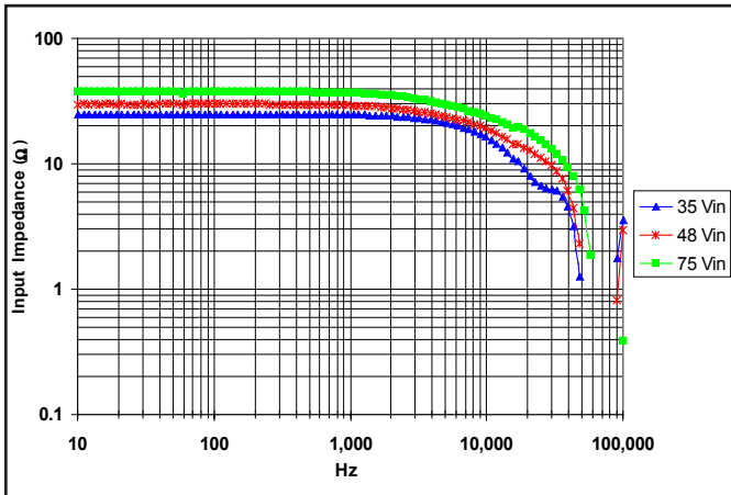
Figure 31: Input impedance ( Z_{in} = V_{in}/I_{in} ) for minimum, nominal, and maximum input voltage at full rated power for 1.5V output.
