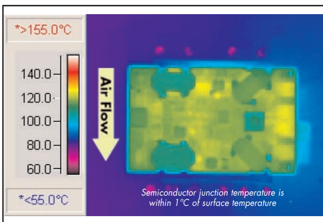
Figure 12: Thermal plot of converter at 12A load on 1.5V output and 9.5A load on 3.3V output with 85°C air flowing at 200 LFM. Air flow across the converter is from pin 1 to pin 3 (nominal input voltage).
