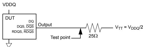
Figure 2 - Slew Rate Test Load
