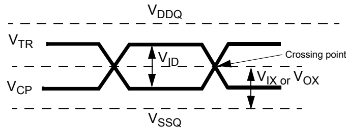
&lt; Differential signal levels &gt;
