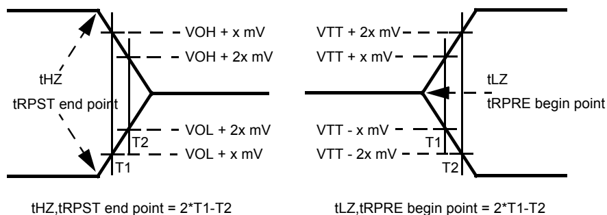
Figure 17 - Method for calculating transitions and endpoints
