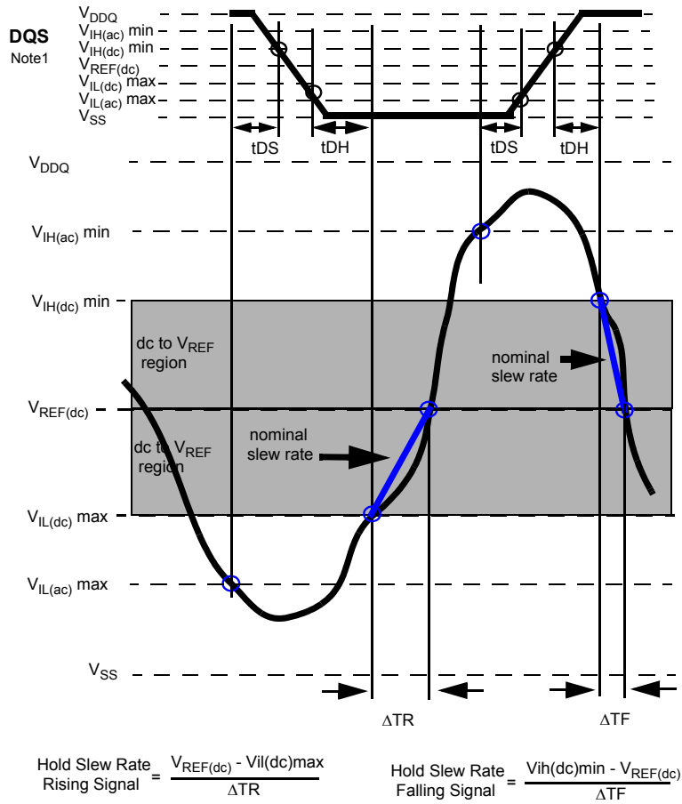
Figure 10 - Illustration of nominal slew rate for tDH (single-ended DQS)
