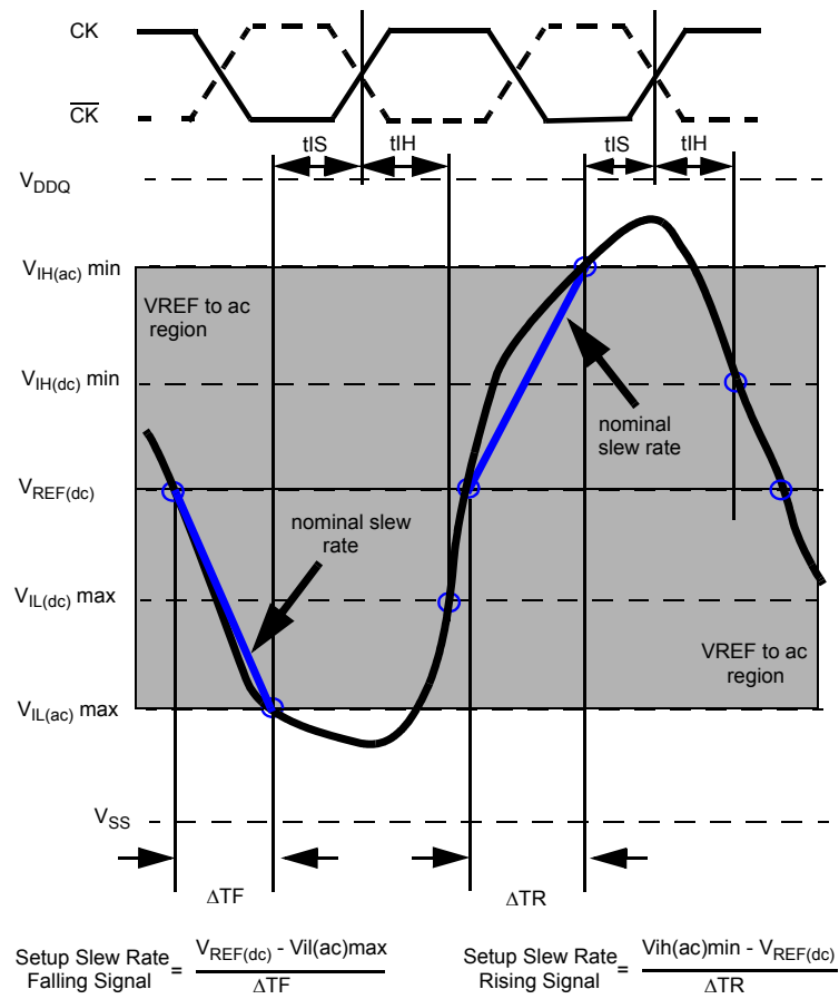
Figure 13 - Illustration of nominal slew rate for tIS
