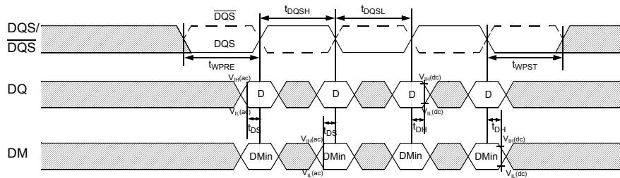
Figure 3 - Data Input (Write) Timing
