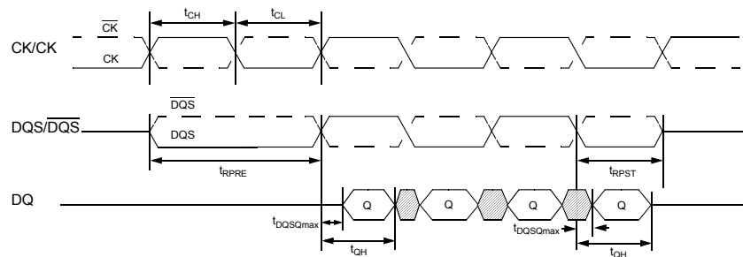
Figure 4 - Data Output (Read) Timing
