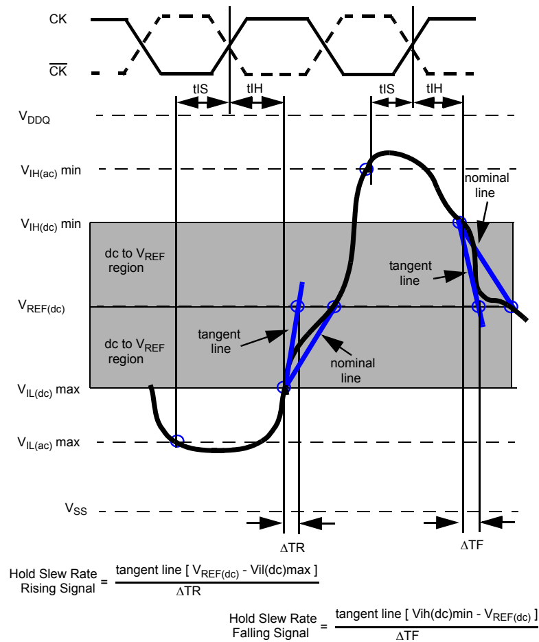
Figure 16 - Illustration of tangent line for t_{IH}
