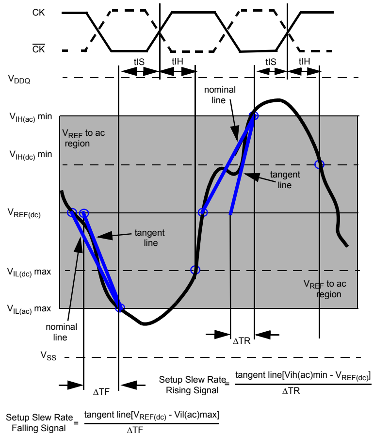
Figure 14 - Illustration of tangent line for tIS
