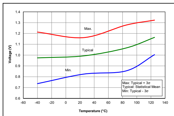
FIGURE 32-73: POR Rearm Voltage, NP Mode, PIC16LF1788/9 Only.
