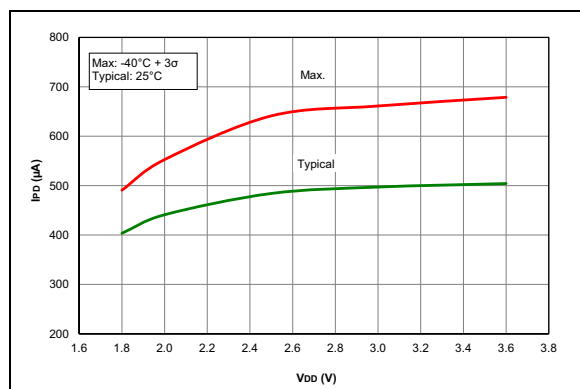
FIGURE 32-49: I_{PO} , Comparator, NP Mode ( C_{XSP} = 1 ), PIC16LF1788/9 Only.
