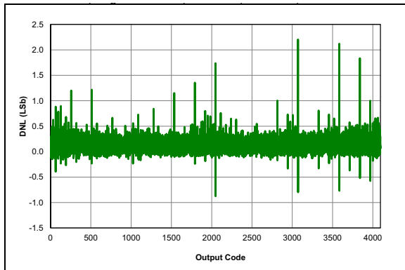
FIGURE 32-93: ADC 12-bit Mode, Single-Ended DNL, V_{DD} = 5.5V , T_{AD} = 1\text{ }\mu S , 25^\circ C .
