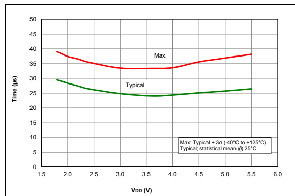
FIGURE 32-75: Wake From Sleep, V_{REGPM} = 1 .
