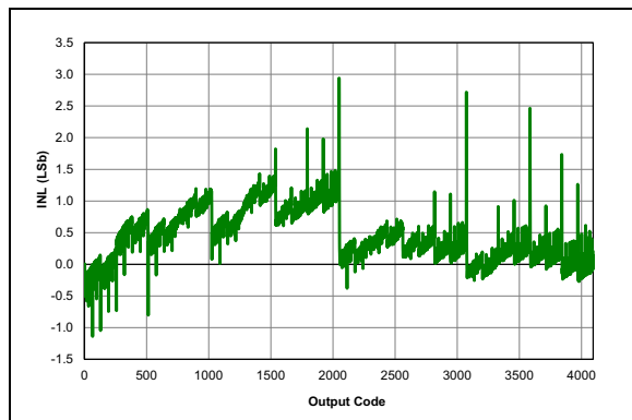
FIGURE 32-87: ADC 12-bit Mode, Single-Ended INL, V_{DD} = 3.0V , T_{AD} = 1\text{ }\mu\text{s} , 25^\circ\text{C} .
