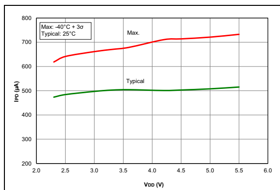
FIGURE 32-50: I_{PO} , Comparator, NP Mode ( C_{XSP} = 1 ), PIC16F1788/9 Only.
