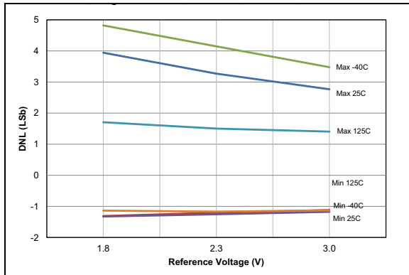
FIGURE 32-91: ADC 12-bit Mode, Single-Ended DNL, V_{DD} = 3.0V , T_{AD} = 1\text{ }\mu S .
