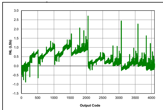
FIGURE 32-88: ADC 12-bit Mode, Single-Ended INL, V_{DD} = 3.0V , T_{AD} = 4\text{ }\mu\text{s} , 25^\circ\text{C} .
