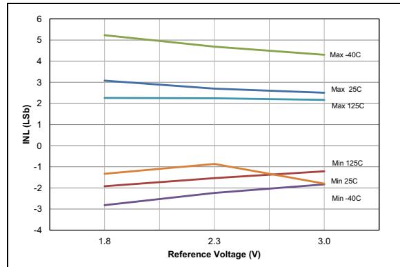
FIGURE 32-92: ADC 12-bit Mode, Single-Ended INL, V_{DD} = 3.0V , T_{AD} = 1\text{ }\mu S .
