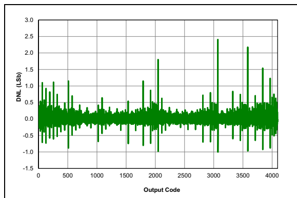
FIGURE 32-85: ADC 12-bit Mode, Single-Ended DNL, V_{DD} = 3.0V , T_{AD} = 1\text{ }\mu\text{s} , 25^\circ\text{C} .
