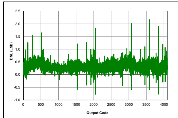
FIGURE 32-94: ADC 12-bit Mode, Single-Ended DNL, V_{DD} = 5.5V , T_{AD} = 4\text{ }\mu S , 25^\circ C .
