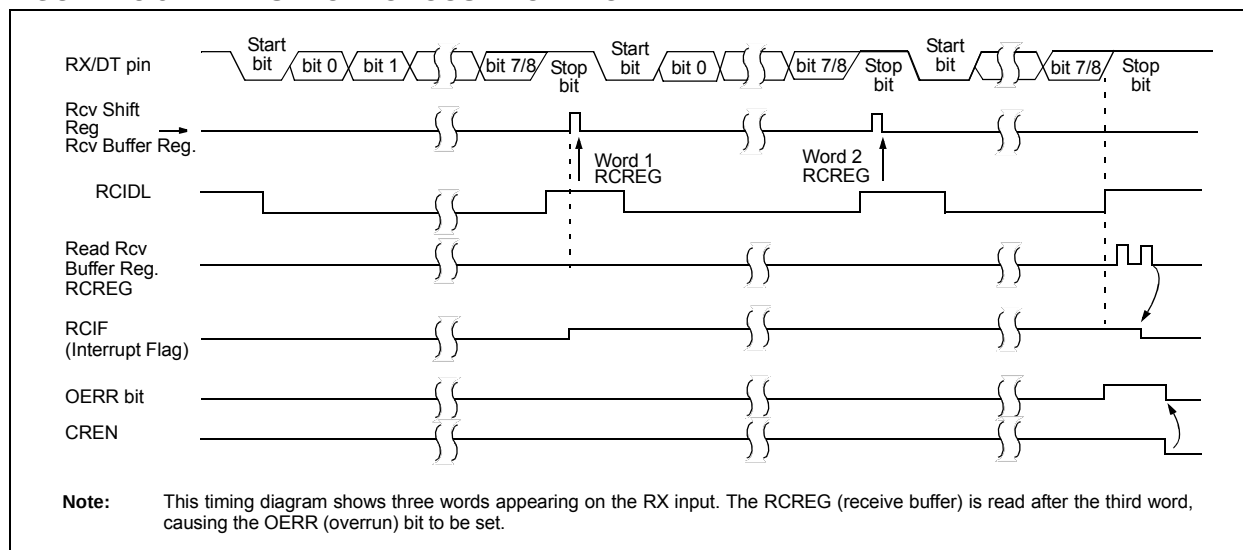
FIGURE 28-5: ASYNCHRONOUS RECEPTION
