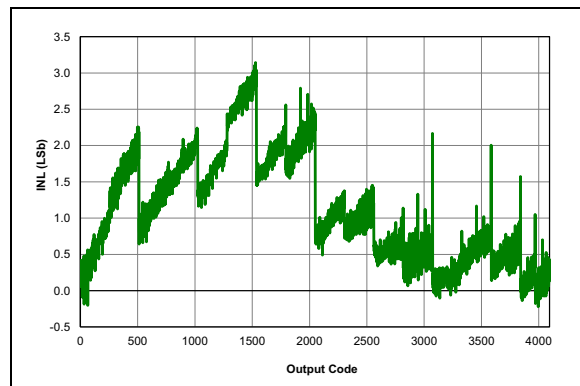
FIGURE 32-96: ADC 12-bit Mode, Single-Ended INL, V_{DD} = 5.5V , T_{AD} = 4\text{ }\mu S , 25^\circ C .
