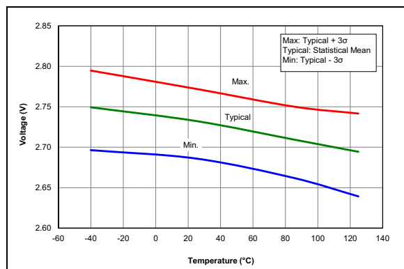
FIGURE 32-65: Brown-Out Reset Voltage, High Trip Point ( BORV = 0 ).
