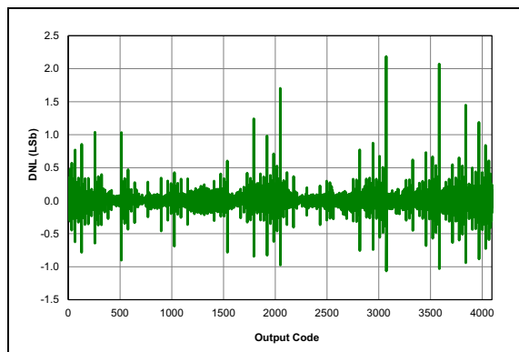
FIGURE 32-86: ADC 12-bit Mode, Single-Ended DNL, V_{DD} = 3.0V , T_{AD} = 4\text{ }\mu\text{s} , 25^\circ\text{C} .
