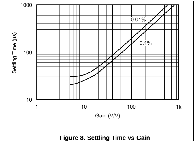
Figure 8. Settling Time vs Gain
