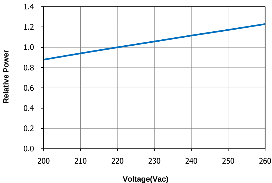
Relative Power Distribution vs. Voltage at Ta=25℃
