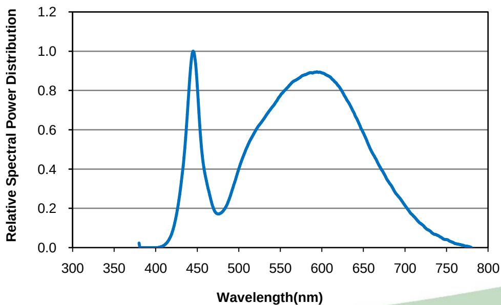
Neutral-White Relative Spectral Power Distribution at Ta=25℃
