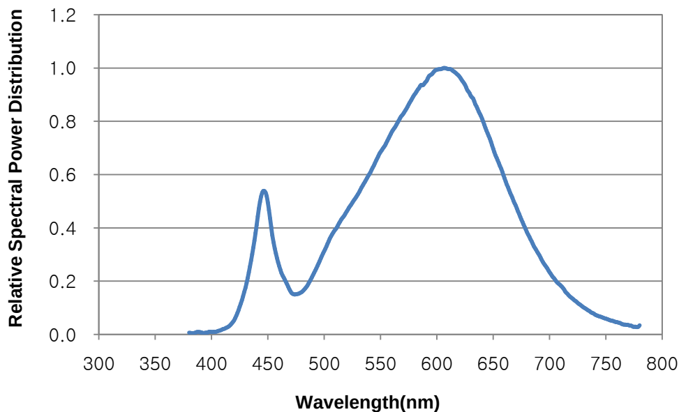
Warm-White Relative Spectral Power Distribution at Ta=25℃
