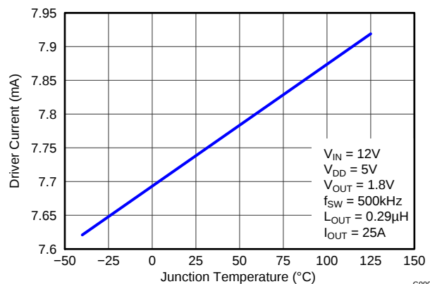
Figure 12. Driver Current vs Temperature
