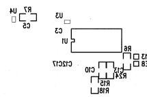
Figure 23. Bottom Silkscreen
