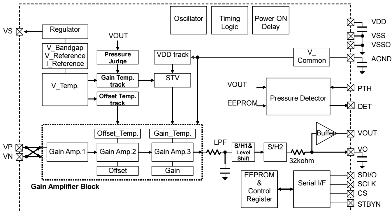
Block Diagram
