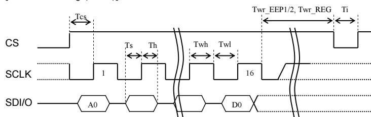
[Serial I/F timing (Write)]
