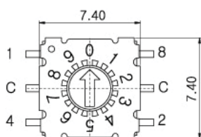
RD81TS SMD Top Type Terminals
