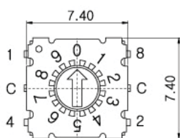
RD81TH THT Top Adjust Type Terminals
