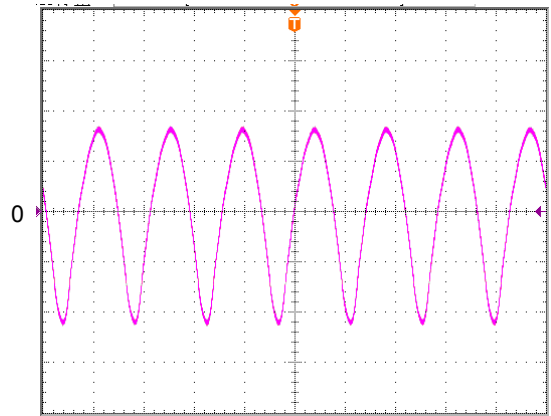
Figure 9: Input Terminal Ripple Current, i_c , at full rated output current and nominal input voltage ( V_{in}=48V ) with 12 \mu H source impedance and 33 \mu F electrolytic capacitor (250mA/div, 2us/div)
