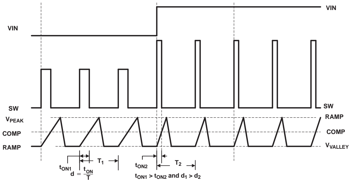
Figure 26. Voltage Feed-Forward and PWM Duty Cycle Waveforms
