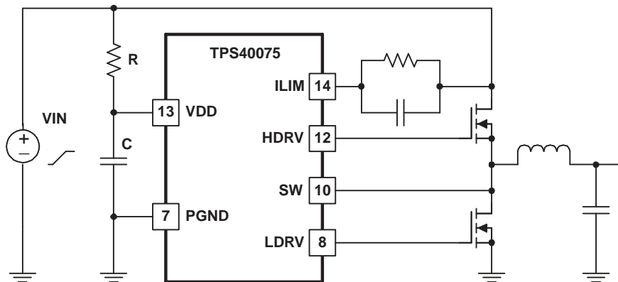
Figure 25. Limiting the Slew Rate
