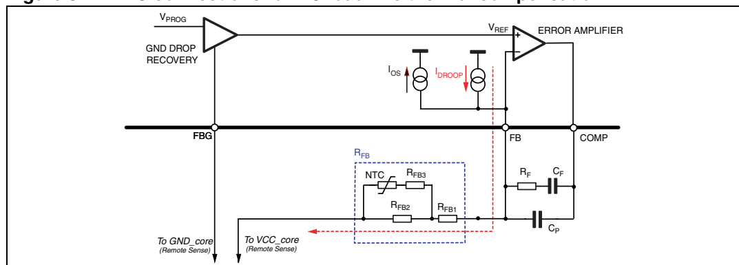
Figure 8. NTC connections for DC load line thermal compensation
