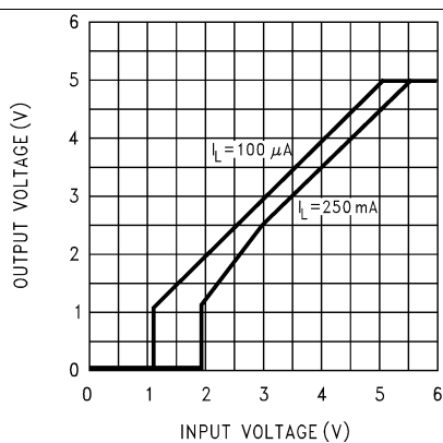
Figure 11. Dropout Characteristics
