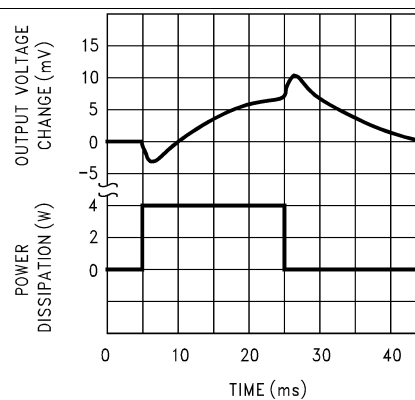
Figure 12. Thermal Response
