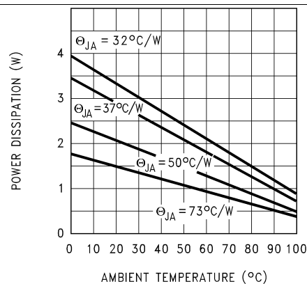
Figure 12. Thermal Response
