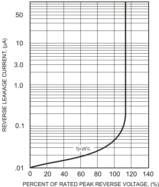
FIG.4-TYPICAL REVERSE CHARACTERISTICS
