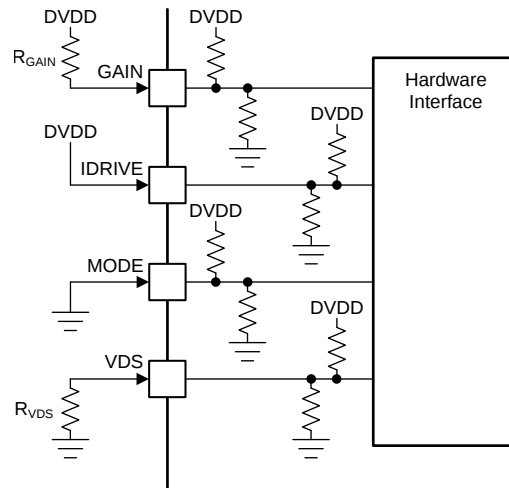
Figure 24. Hardware Interface
