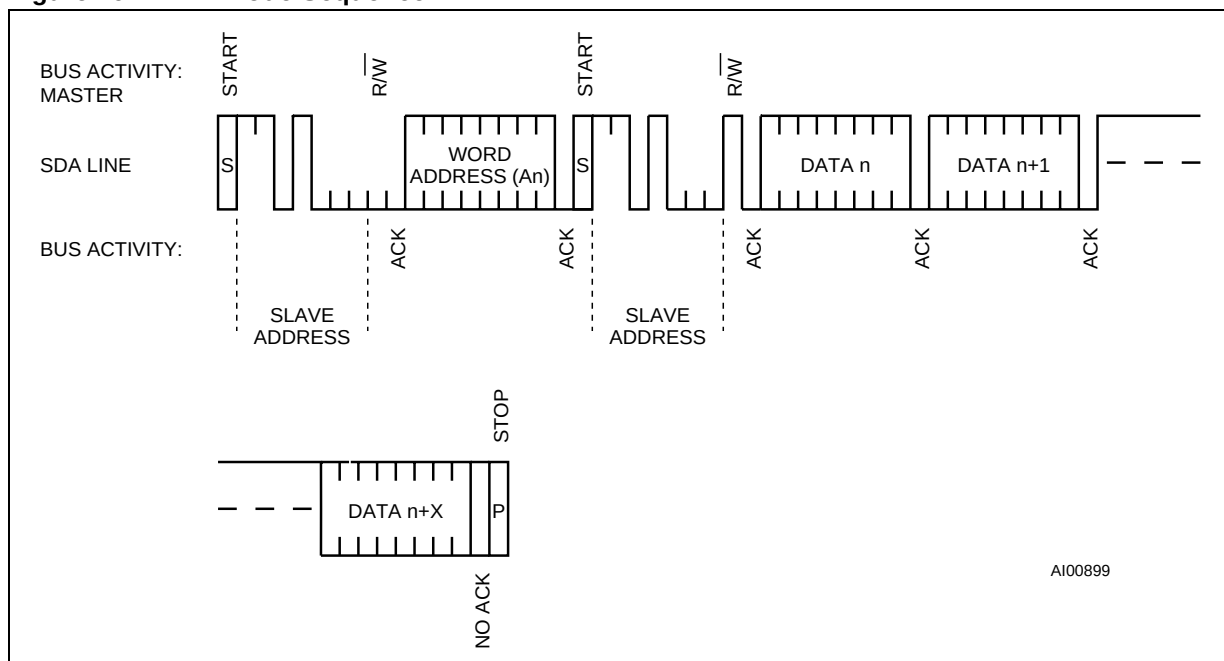
Figure 19. READ Mode Sequence
