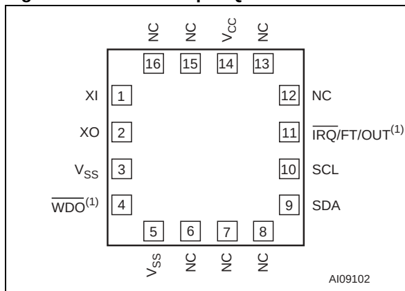
Figure 10. M41T65 16-pin QFN Connections
