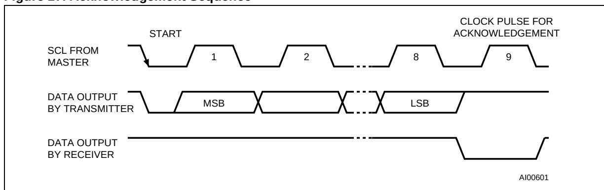
Figure 17. Acknowledgement Sequence
