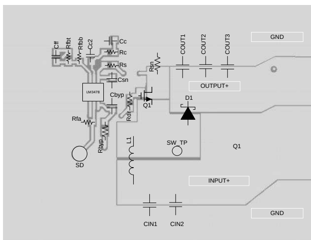
Figure 38. Typical Layout for a Boost Converter
