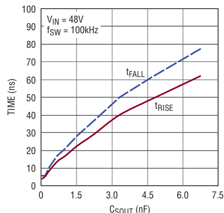
SOUT Driver Transition Time vs Capacitance
