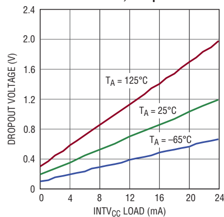
INTV CC Dropout Voltage vs Load Current, Temperature
