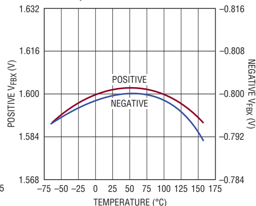
FBX Regulation Voltage vs Temperature
