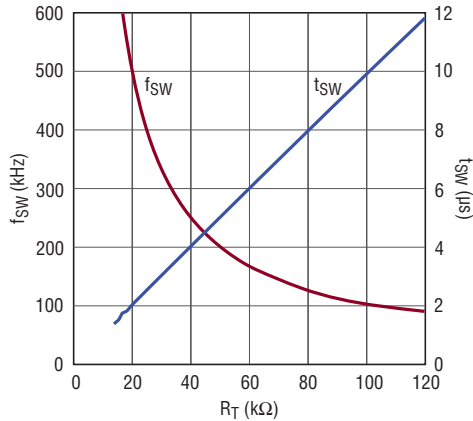
Switching Frequency and (Period) vs Programming Resistance
