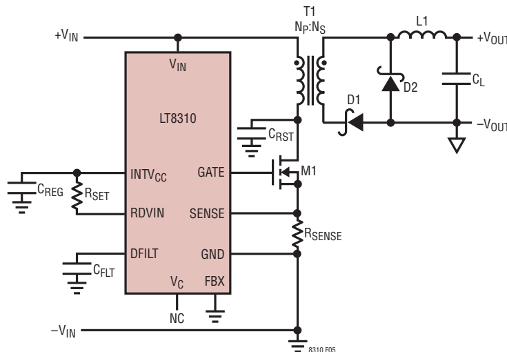
Figure 5. Forward Nonsynchronous Converter Core Schematic
