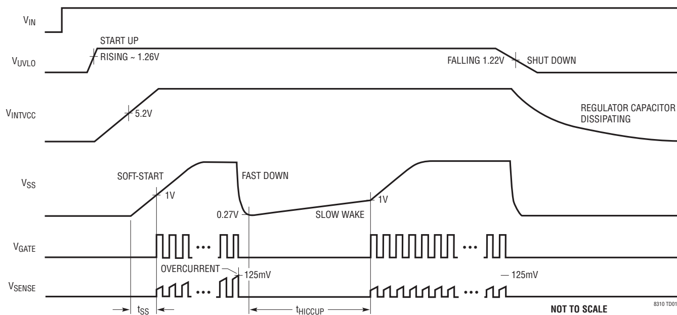
Start-Up/Soft-Start/Fault/Shutdown/Restart
