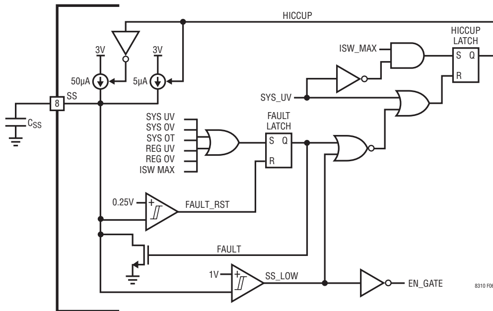
Figure 6. Soft-Start Control Logic
