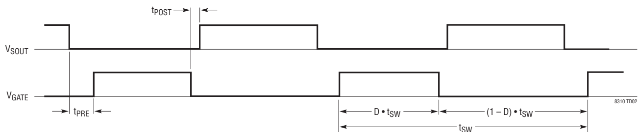
Nonoverlapping GATE/SOUT
