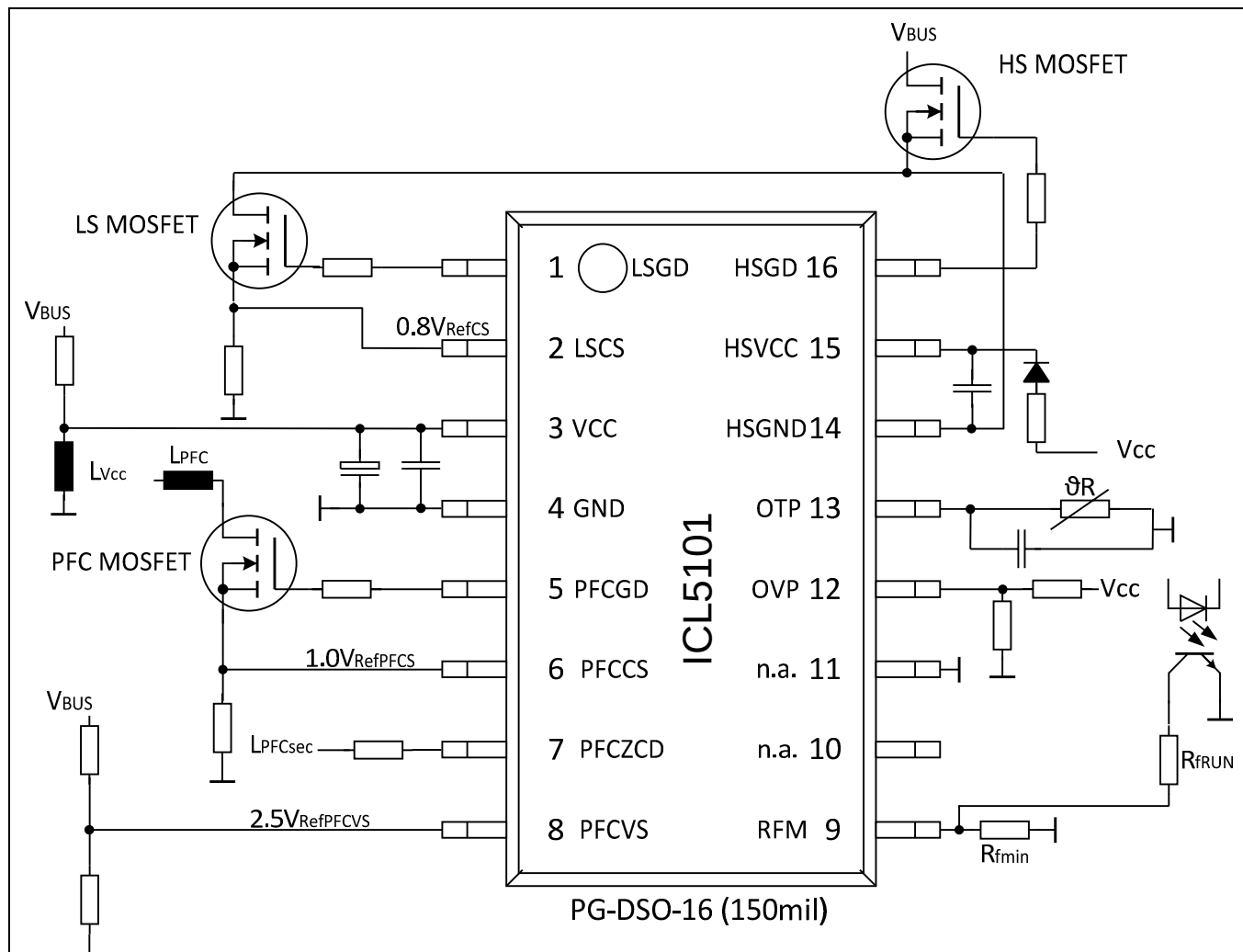
Figure 3 PIN Set-Up
