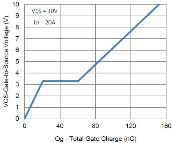
7. Gate Charge
