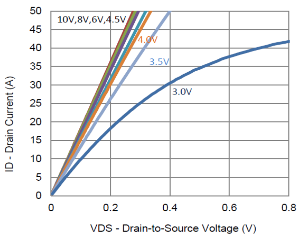
5. Output Characteristics
