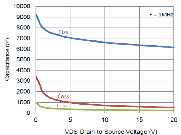
6. Capacitance
