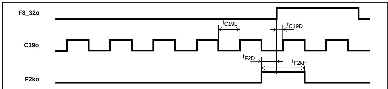
Figure 31 - SDH Output Timing Referenced to F8/F32o
