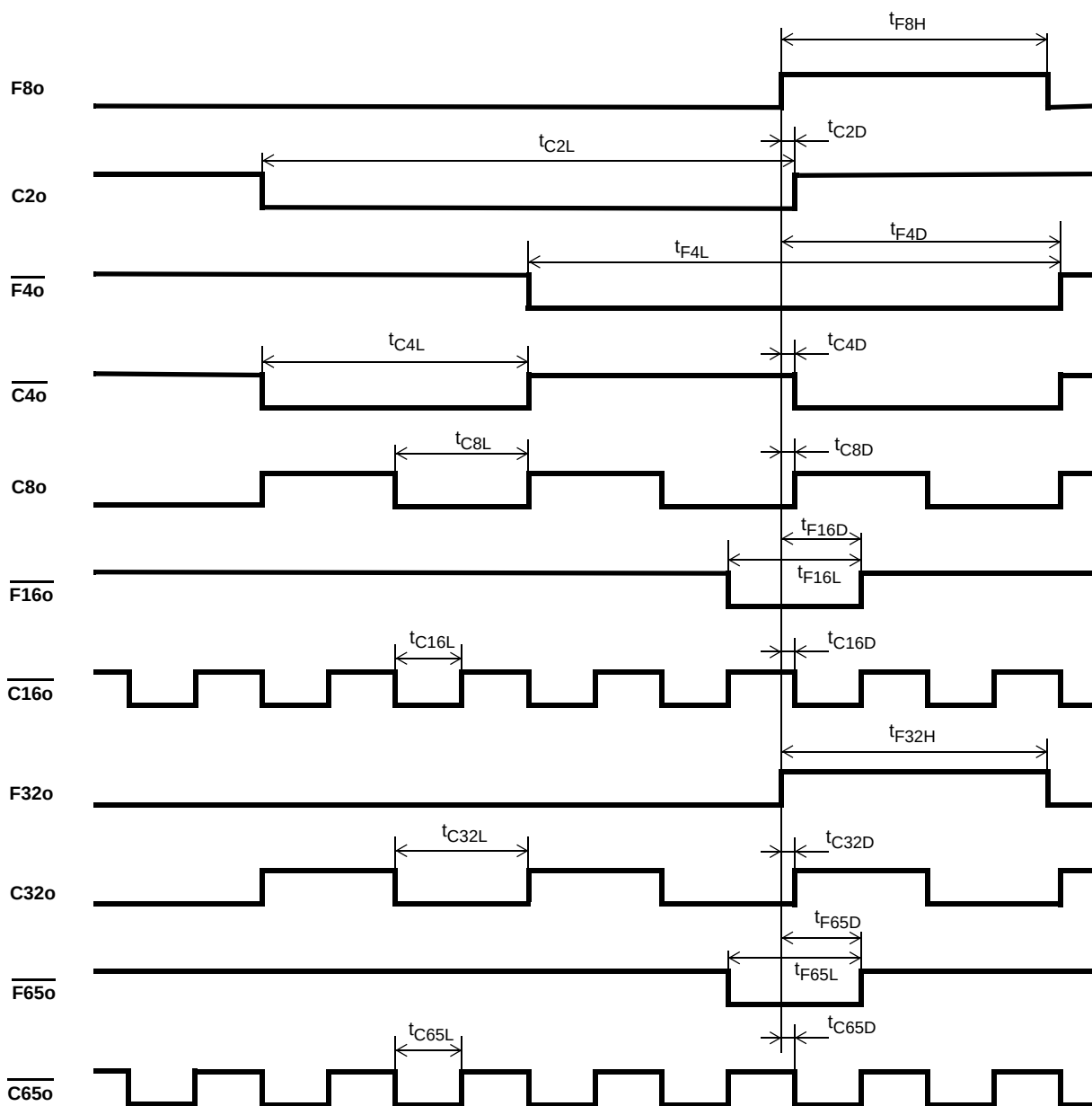
Figure 29 - E1 Output Timing Referenced to F8/F32o
