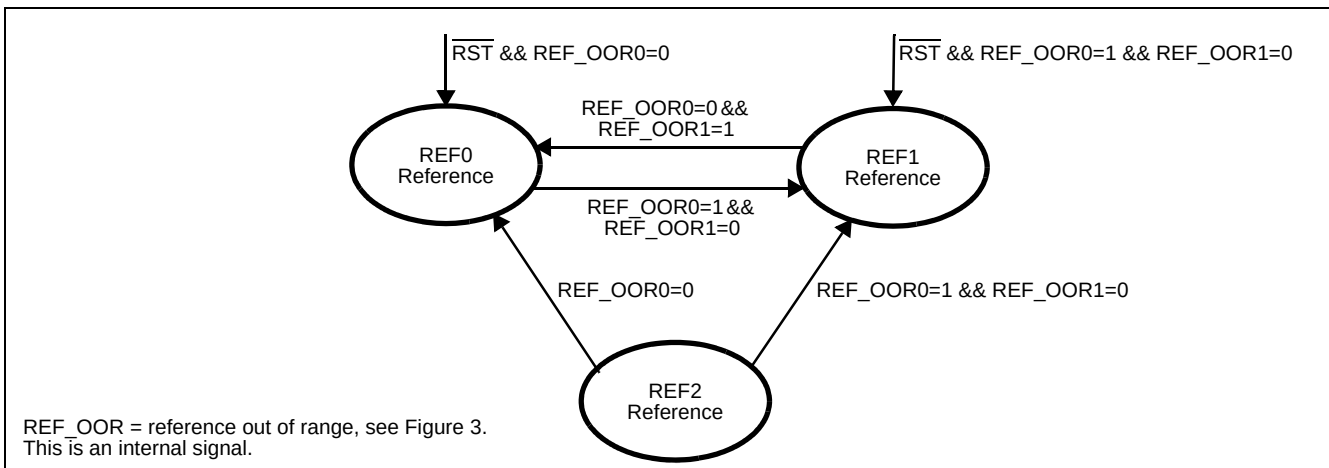
Figure 14 - Reference Selection in Automatic Mode ( \text{MODE\_SEL}=11 )
