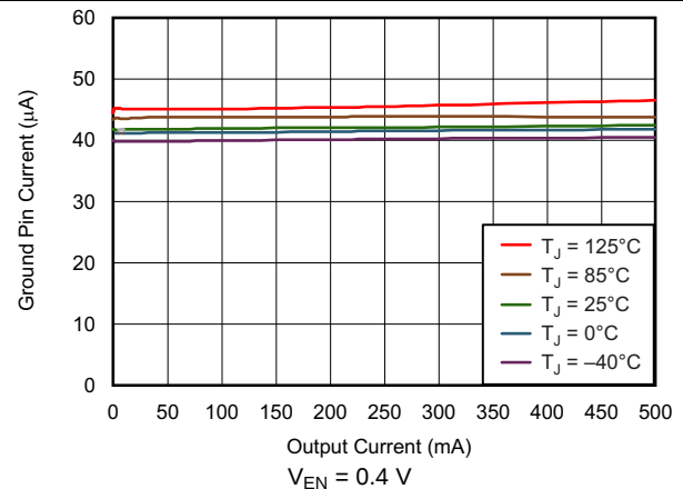
Figure 6. TPS73525 Ground Pin Current (Disable) vs Temperature
