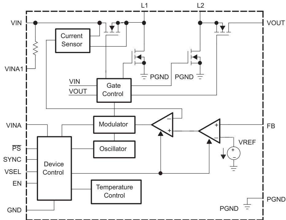
FUNCTIONAL BLOCK DIAGRAM (TPS63011, TPS63012)
