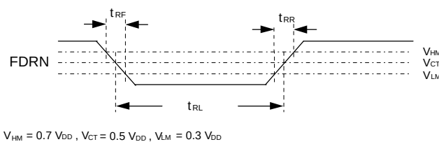
Figure 8-5. FDRN Output Timing
