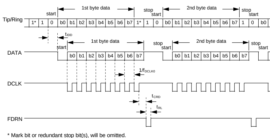
Figure 8-6. Serial Data Interface Timing of FSK Demodulation in Mode 0
