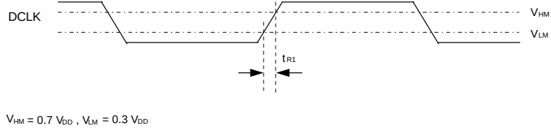
Figure 8-7. DCLK Mode 1 Input Timing
