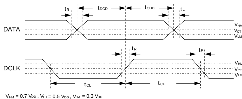
Figure 8-4. Data and DCLK Mode 0 Output Timing
