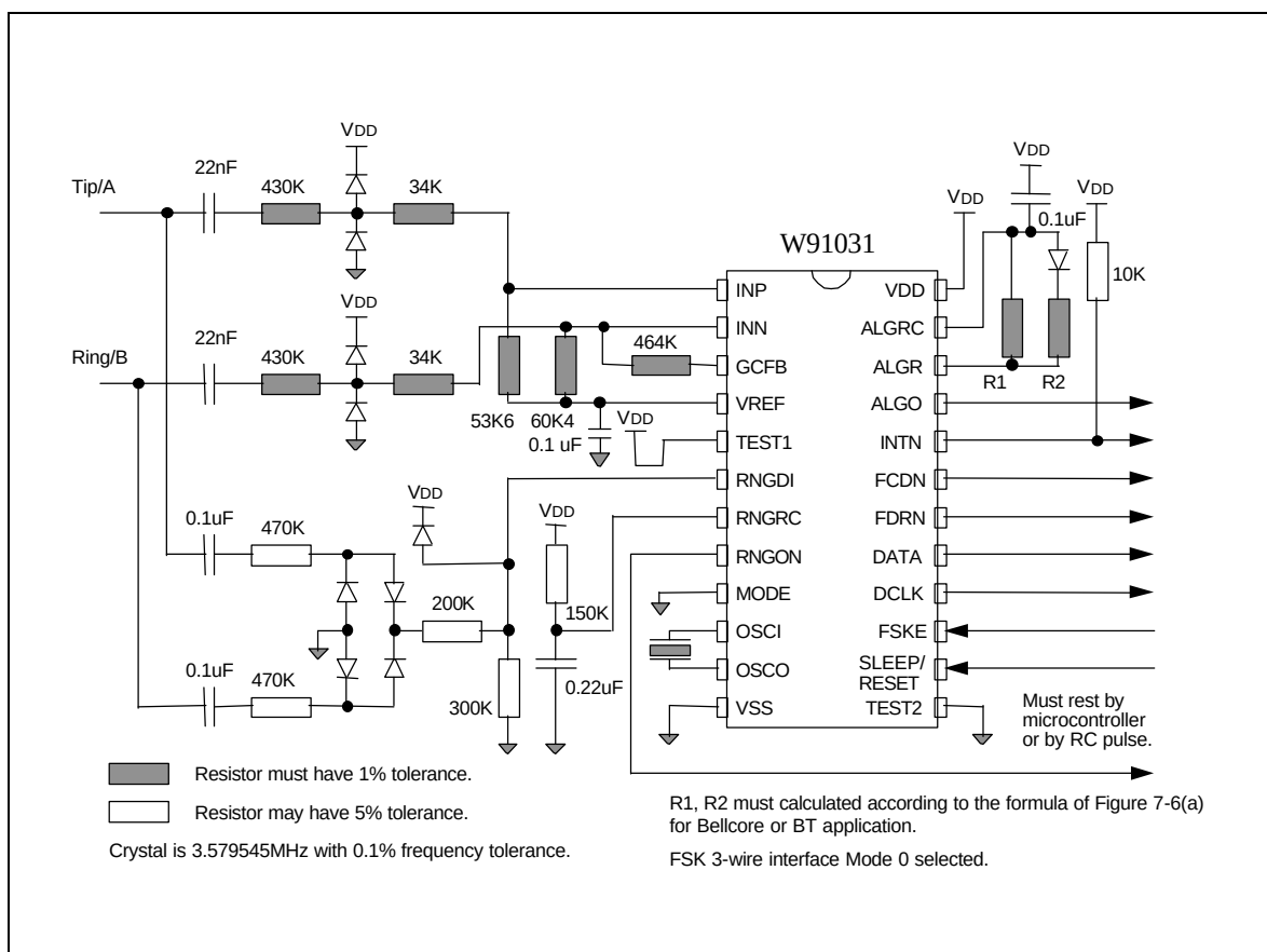
Figure 9-1. Application Circuit.
