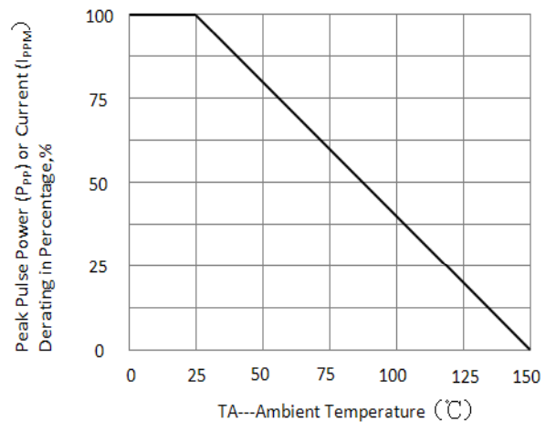
Figure 4. Peak Pulse Power Derating Curve
