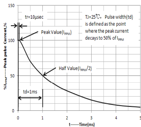
Figure 3. Pulse Waveform
