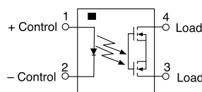
CPC1016N Pinout
