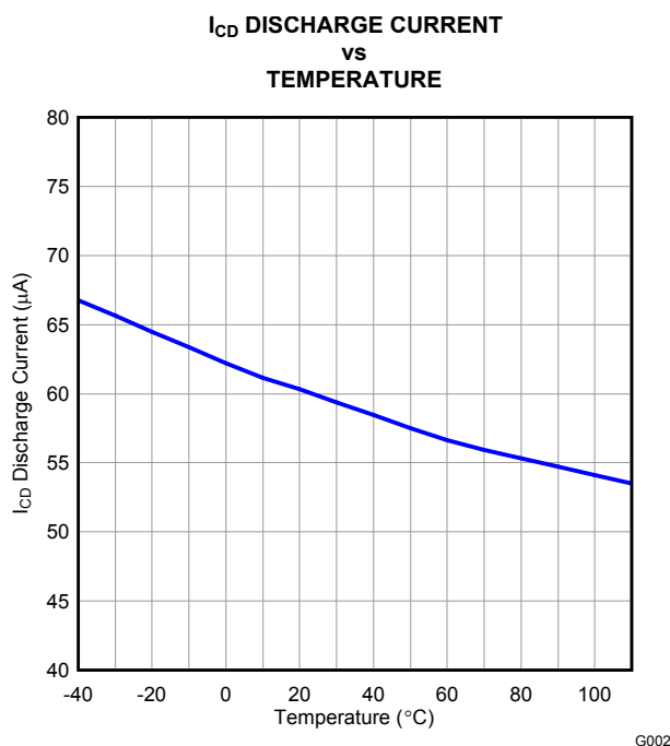
Figure 2. I_{CD} Discharge Current
