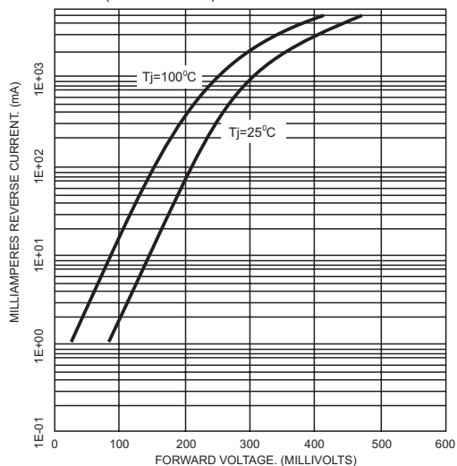
FIG.5- TYPICAL FORWARD CHARACTERISTICS (FOR SKL22A)
