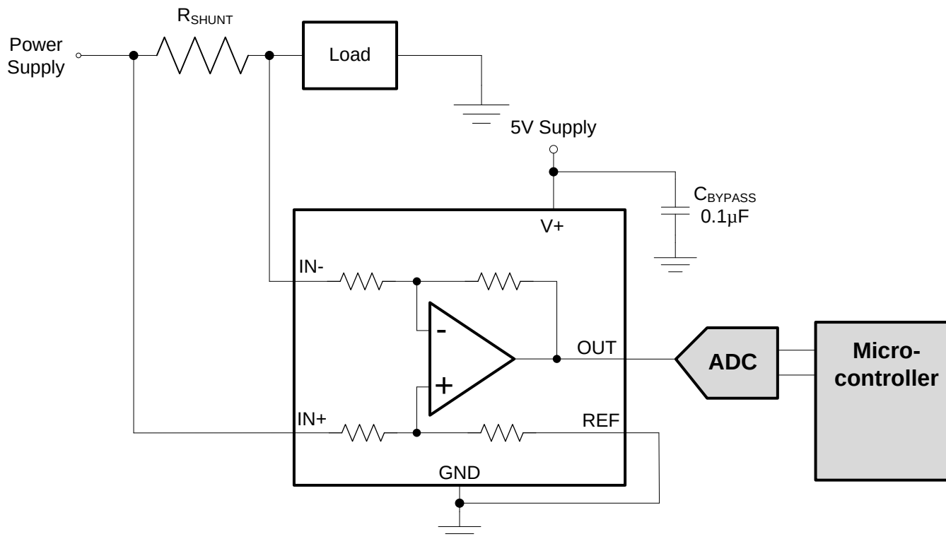
Figure 23. Typical Application
