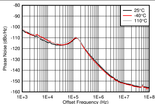
Figure 6-616. Phase Noise for 10-GHz VCO at 5 MHz vs Temperature and f_{REF} at f_{OUT} = 2.6 GHz
