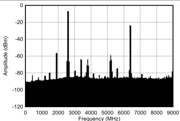
Figure 6-427. TX Single Tone (-1 dBFS) Output Spectrum at 2.6 GHz ( 0 - f_{\text{DAC}} )
