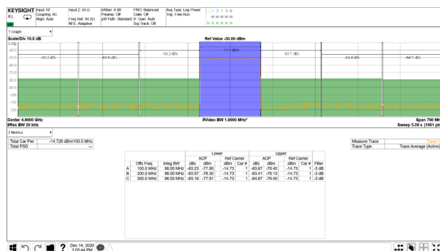
Figure 6-528. TX 100-MHz NR Output Spectrum at 4.9 GHz
