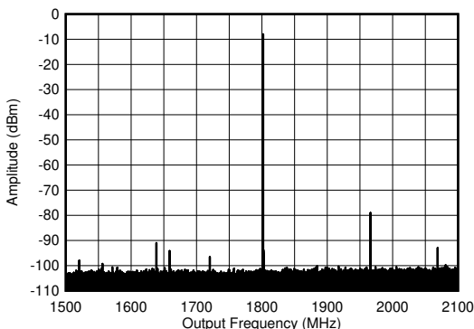
f_{\text{DAC}} = 8847.36\text{ MSPS} , interleave mode, 1.8 GHz matching, includes PCB and cable losses Figure 6-364. TX Single Tone (-6 dBFS) Output Spectrum at 1.8 GHz ( \pm 300\text{ MHz} )
