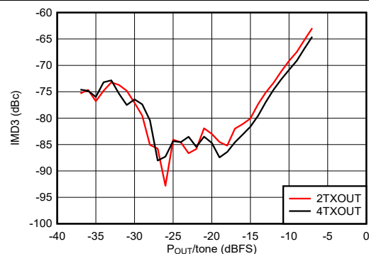
Figure 6-526. TX IMD3 vs Digital Level at 4.9 GHz
