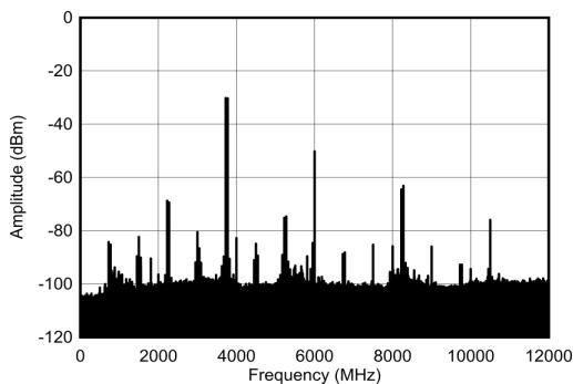
Figure 6-495. TX Dual Tone Output Spectrum at 3.75 GHz, -13 dBFS each (0 - f_{\text{DAC}} )
