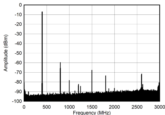
Figure 6-282. Dual Tone Spectrum at 400 MHz and -13 dBFS (Nyquist)
