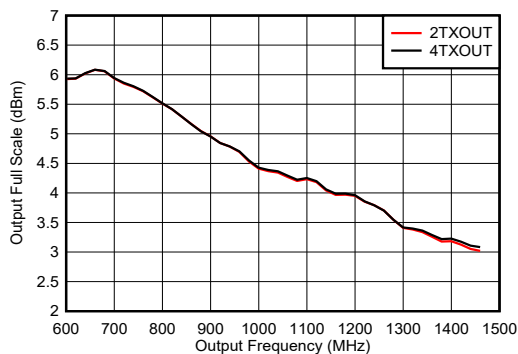
Figure 6-296. TX Full Scale vs RF Frequency and Channel at 5898.24 MSPS, Interleave Mode
