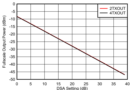
Figure 6-548. TX Full Scale vs DSA Setting and Channel at 7.1 GHz
