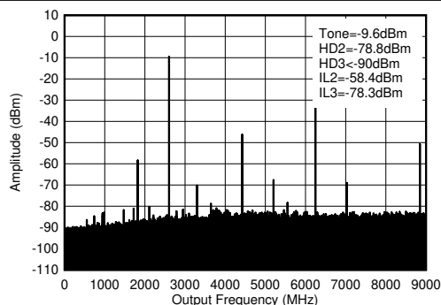
Figure 6-415. Two Tone Inband SFDR vs Digital Amplitude at 2.6 GHz
