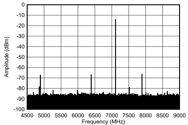
Figure 6-581. Single Tone Output Spectrum at 7.1 GHz, -6 dBFS (Nyquist)
