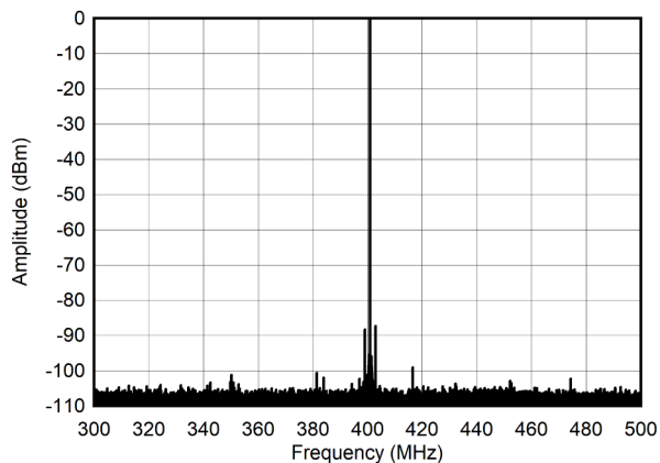
Figure 6-273. Single Tone Spectrum at 400 MHz and -6 dBFS (±100MHz)
