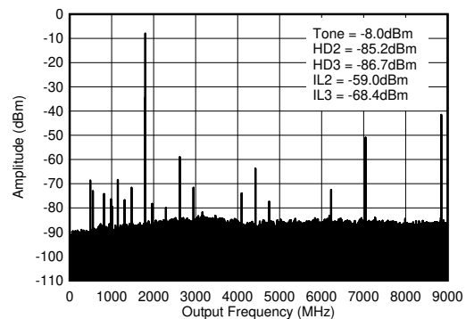
f_{\text{DAC}} = 8847.36\text{ MSPS} , interleave mode, 1.8 GHz matching, includes PCB and cable losses. \text{ILn} = f_s/n \pm f_{\text{OUT}} . Figure 6-363. TX Single Tone (-12 dBFS) Output Spectrum at 1.8 GHz ( 0-f_{\text{DAC}} )
