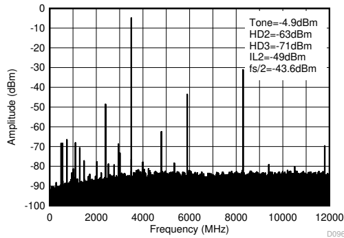
Figure 6-489. TX Single Tone (-6 dBFS) Output Spectrum at 3.5 GHz (0- f_{\text{DAC}} )
