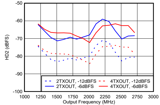
Matching at 1.8 GHz, f_{\text{DAC}} = 11.79648\text{ GSPS} , interleave mode, normalized to output power at harmonic frequency Figure 6-361. TX HD2 vs Digital Amplitude and Output Frequency at 1.8 GHz
