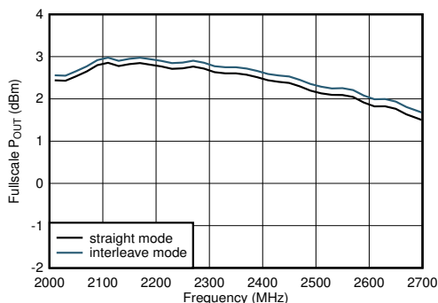
Figure 6-375. TX Full Scale vs RF Frequency at 5898.24 MSPS
