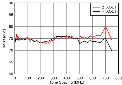
Figure 6-570. IMD3 vs Tone Spacing and Channel at 7.1 GHz
