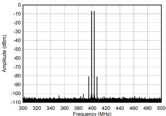
Figure 6-283. Dual Tone Spectrum at 400 MHz and -13 dBFS (±100MHz)
