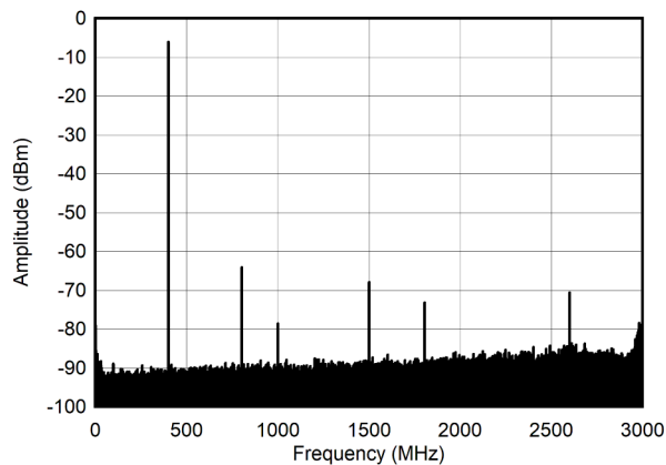
Figure 6-274. Single Tone Spectrum at 400 MHz and -12 dBFS (Nyquist)
