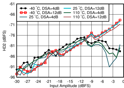
Figure 6-72. RX HD2 vs Input Level and Temperature at 0.8 GHz
