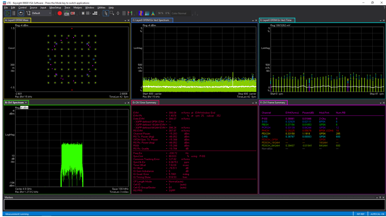
Figure 6-545. TX 20-MHz LTE Error Vector Magnitude at 4.9 GHz
