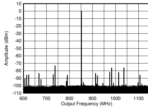
Figure 6-345. TX Single Tone (-6 dBFS) Output Spectrum at 0.85 GHz ( \pm 300 MHz)
