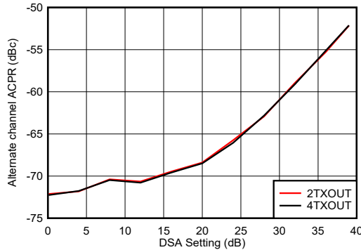
Matching at 1.8 GHz, single carrier 20-MHz BW TM1.1 LTE Figure 6-360. TX 20-MHz LTE alt-ACPR vs DSA at 1.8 GHz
