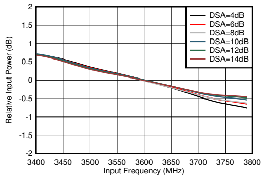
Figure 6-137. RX In-Band Gain Flatness, f_{\text{IN}} = 3600 \text{ MHz}
