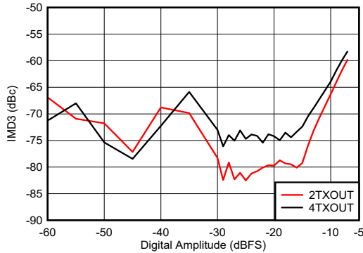
Figure 6-439. IMD3 vs Digital Amplitude and Channel at 2.6 GHz
