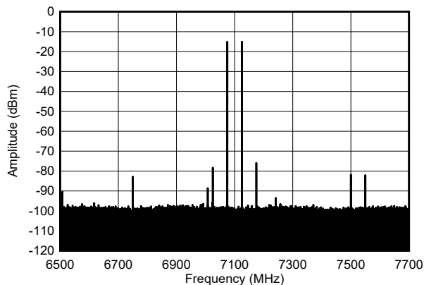
Figure 6-586. Two Tone Output Spectrum at 7.1 GHz, -7 dBFS each (narrow band)
