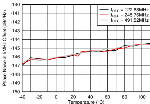
Figure 6-616. Phase Noise for 10-GHz VCO at 5 MHz vs Temperature and f_{REF} at f_{OUT} = 2.6 GHz
