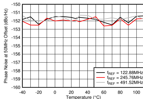
Figure 6-617. Phase Noise for 10-GHz VCO at 50 MHz vs Temperature and f_{REF} at f_{OUT} = 2.6 GHz
