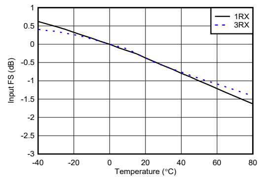
Figure 6-174. RX Input Fullscale vs Temperature and Channel at 4.9 GHz
