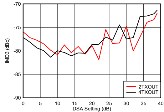
Figure 6-523. TX IMD3 vs DSA Setting at 4.9 GHz
