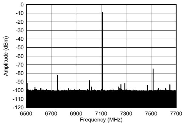
Figure 6-580. Single Tone Output Spectrum at 7.1 GHz, -1 dBFS (narrow span)
