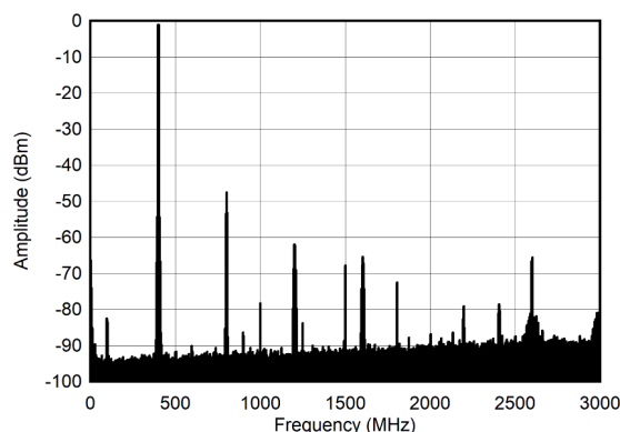
Figure 6-280. Dual Tone Spectrum at 400 MHz and -7 dBFS (Nyquist)
