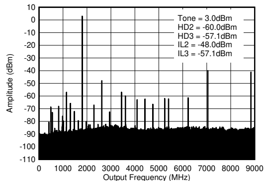
Figure 6-367. TX Single Tone (-1 dBFS) Output Spectrum at 1.8 GHz ( 0-f_{\text{DAC}} )
