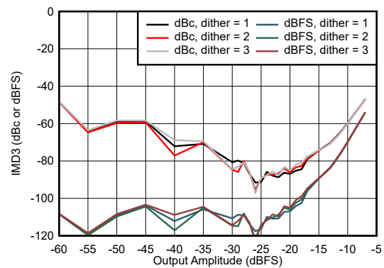
Figure 6-256. IMD3 vs Digital Amplitude at 30 MHz
