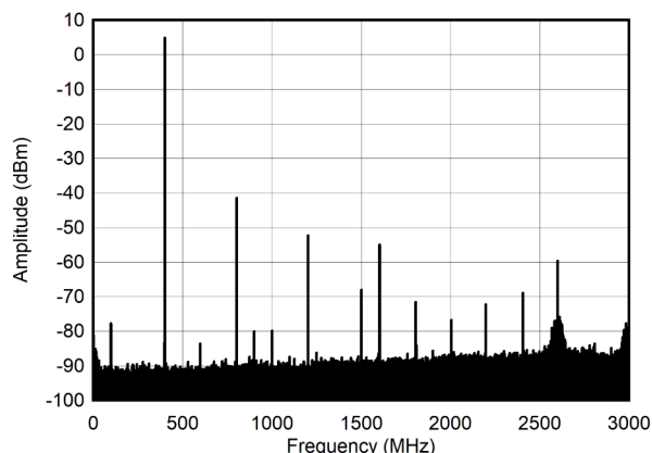
Figure 6-270. Single Tone Spectrum at 400 MHz and -1 dBFS (Nyquist)
