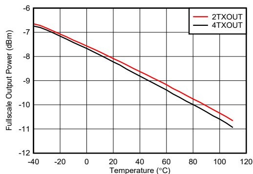
Figure 6-547. TX Full Scale vs Temperature and Channel at 7.1 GHz
