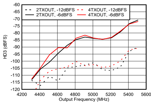
Figure 6-538. TX HD3 vs Digital Amplitude and Output Frequency at 4.9 GHz
