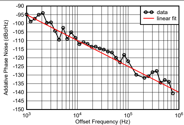
Figure 6-593. RX Additive Phase Noise at 9.61GHz
