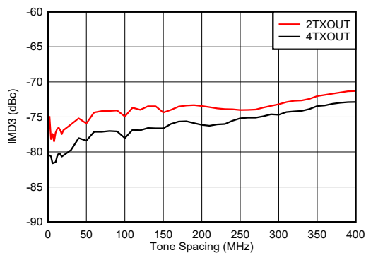
Figure 6-320. TX IMD3 vs Tone Spacing and Channel at 0.85 GHz
