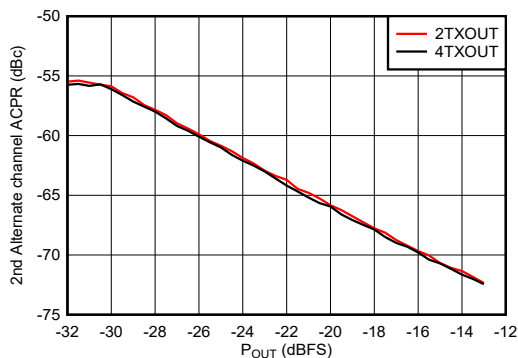
Figure 6-356. TX 20-MHz LTE ACPR vs Digital Level at 1.8425 GHz
