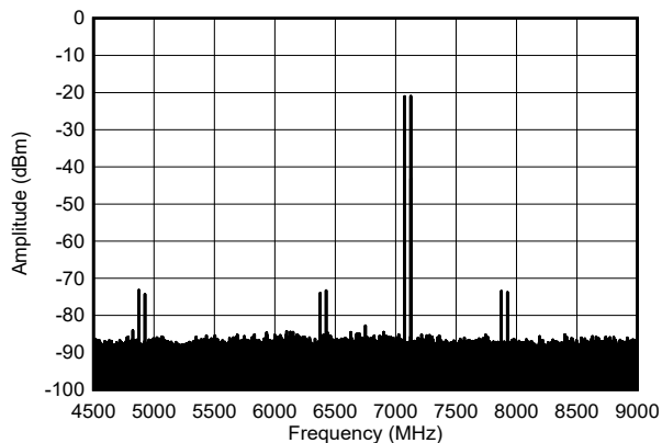
Figure 6-585. Two Tone Output Spectrum at 7.1 GHz, -7 dBFS each (Nyquist)
