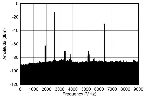
Figure 6-429. TX Dual Tone Output Spectrum at 2.6 GHz, -7 dBFS each ( 0 - f_{\text{DAC}} )
