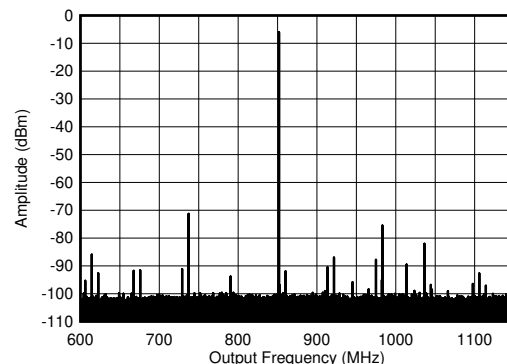
Figure 6-347. TX Single Tone (-1 dBFS) Output Spectrum at 0.85 GHz ( \pm 300 MHz)
