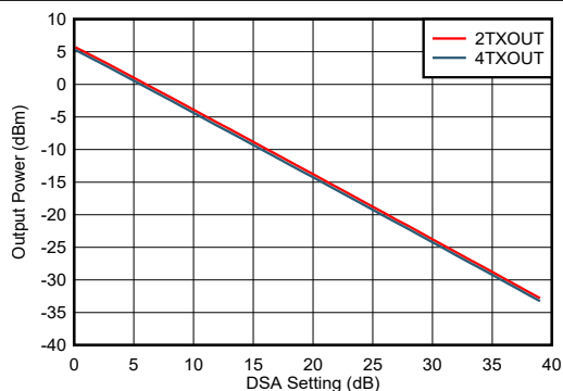
Figure 6-261. TX Output Fullscale vs DSA Setting at 400 MHz
