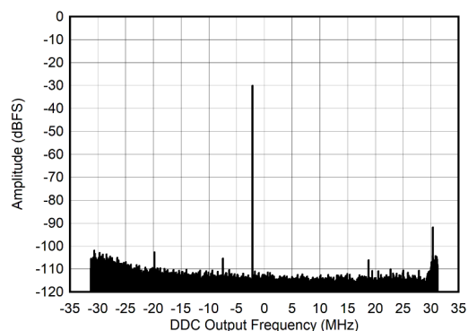
Figure 6-16. RX Output FFT at 30 MHz
