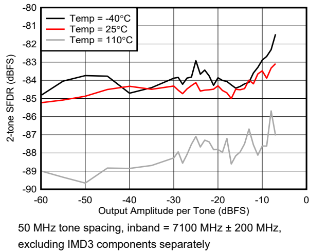
Figure 6-578. Two Tone Inband SFDR vs Output Amplitude at 7.1 GHz
