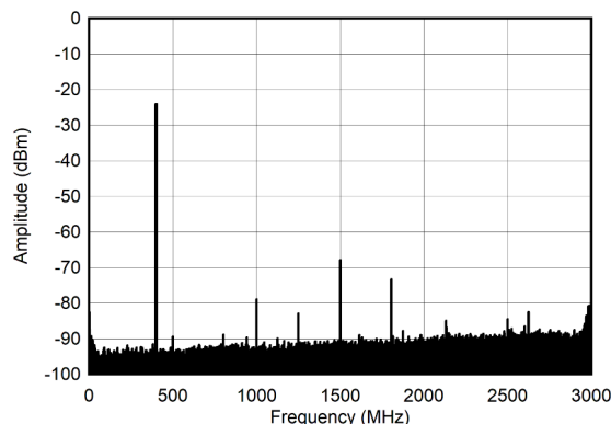
Figure 6-284. Dual Tone Spectrum at 400 MHz and -30 dBFS (Nyquist)
