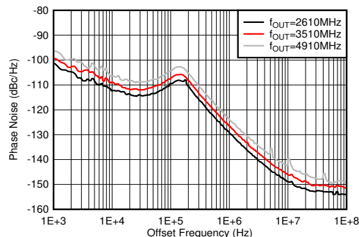
Figure 6-619. Phase Noise for 9-GHz VCO vs Offset Frequency and f_{OUT} at 25°C
