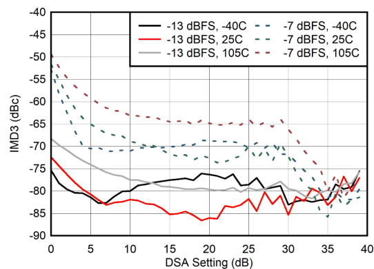
Figure 6-291. IMD3 vs DSA Setting at 400 MHz
