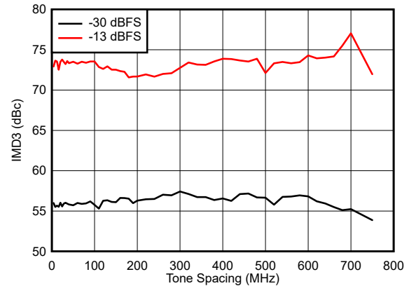
Figure 6-571. IMD3 vs Tone Spacing and Digital Amplitude at 7.1 GHz
