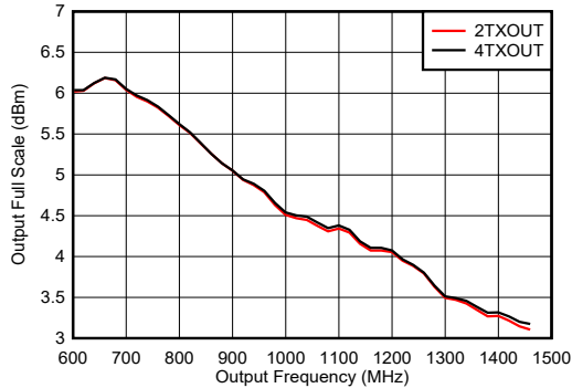
Figure 6-294. TX Full Scale vs RF Frequency and Channel at 5898.24 MSPS, Straight Mode
