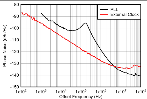
Figure 6-592. Phase Noise vs Offset Frequency for PLL and External Clock at 12GHz
