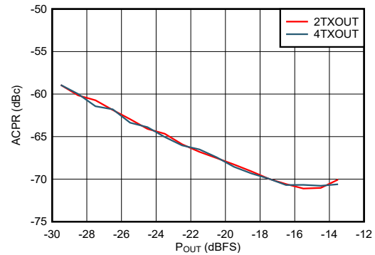
Figure 6-404. TX 20-MHz LTE ACPR vs Digital Level at 2.6 GHz
