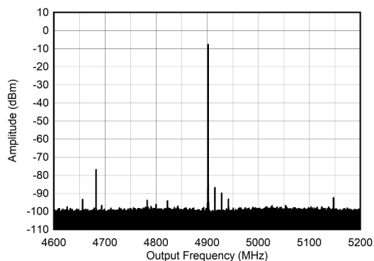
Figure 6-540. TX Single Tone (–1 dBFS) Output Spectrum at 4.9 GHz (±300 MHz)
