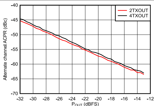
Figure 6-530. TX 20-MHz LTE alt-ACPR vs Digital Level at 4.9 GHz
