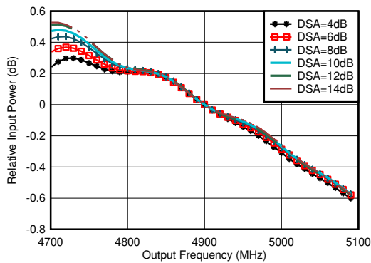
Figure 6-173. RX Inband Gain Flatness, f_{\text{IN}} = 4900 \text{ MHz}
