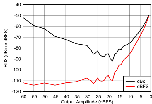
Figure 6-293. HD3 vs Amplitude at 400 MHz
