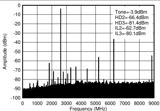
Figure 6-423. TX Single Tone (-12 dBFS) Output Spectrum at 2.6 GHz ( 0-f_{\text{DAC}} )
