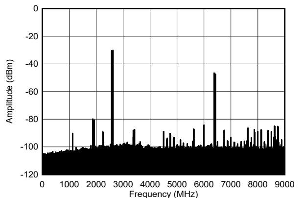
Figure 6-433. TX Dual Tone Output Spectrum at 2.6 GHz, -30 dBFS each (0 - DAC)
