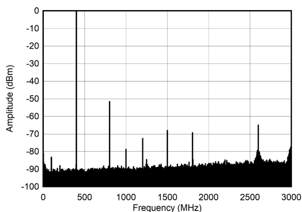
Figure 6-272. Single Tone Spectrum at 400 MHz and -6 dBFS (Nyquist)
