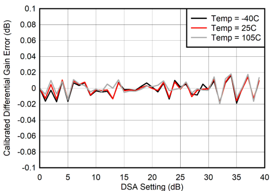
Figure 6-263. Calibrated TX Differential Gain Error (DNL) at 400 MHz
