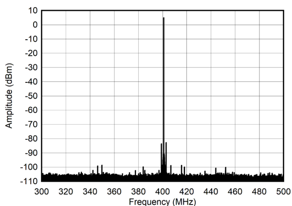
Figure 6-271. Single Tone Spectrum at 400 MHz and -1 dBFS (±100MHz)
