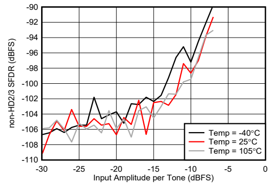
Figure 6-221. RX 2-tone SFDR vs Input Amplitude at 6.85 GHz
