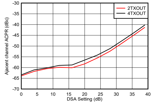
Figure 6-535. TX 100-MHz NR ACPR vs DSA at 4.9 GHz
