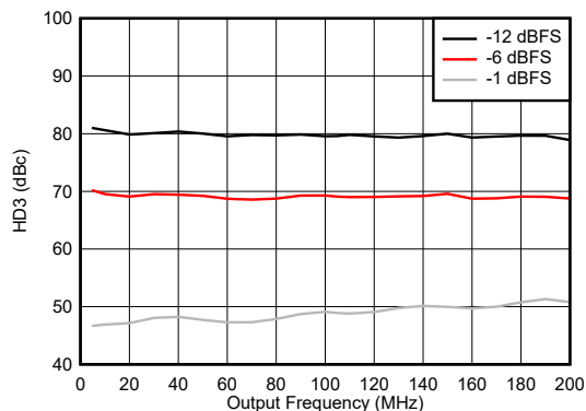
Figure 6-259. HD3 vs Frequency 0 - 200 MHz
