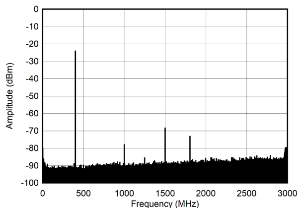
Figure 6-276. Single Tone Spectrum at 400 MHz and -30 dBFS (Nyquist)
