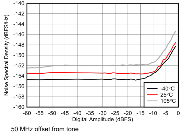
Figure 6-577. NSD vs Digital Amplitude and Temperature at 7.1 GHz
