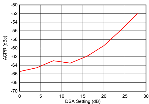
Figure 6-334. TX 20-MHz LTE ACPR vs DSA at 0.85 GHz
