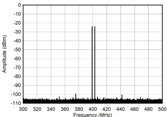
Figure 6-285. Dual Tone Spectrum at 400 MHz and -30 dBFS (±100MHz)
