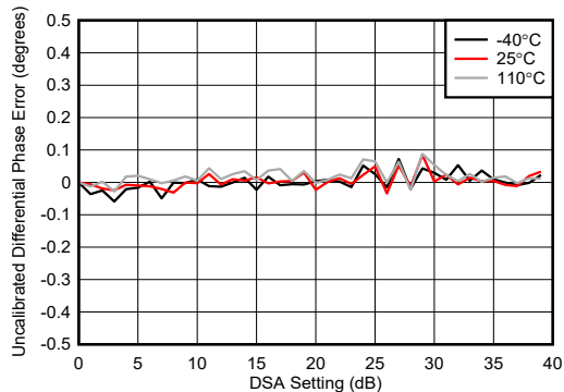
Figure 6-558. Uncalibrated Differential Phase Error vs Temperature at 7.1 GHz
