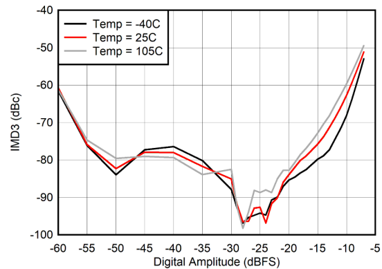
Figure 6-290. IMD3 vs Digital Amplitude at 400 MHz
