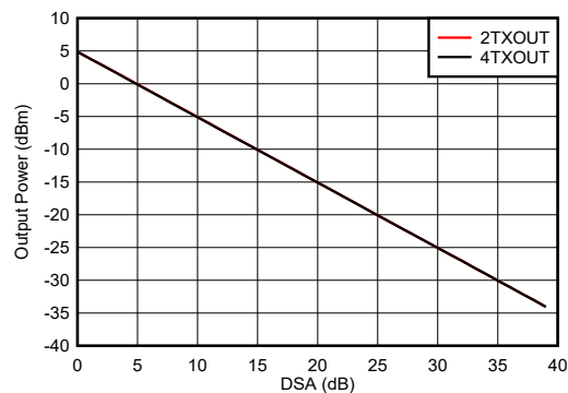
Figure 6-301. TX Output Power vs DSA Setting and Channel at 0.85 GHz
