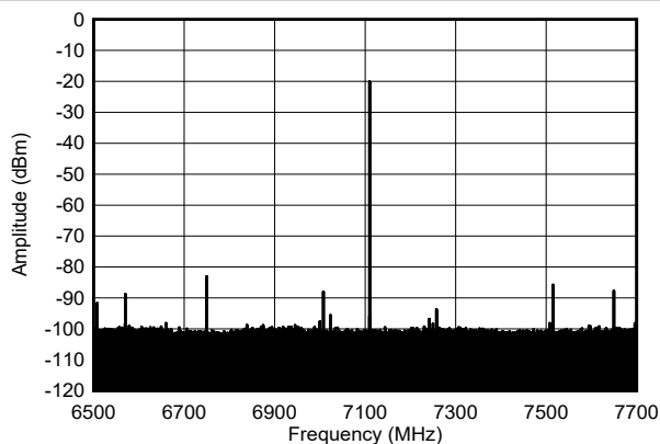
Figure 6-584. Single Tone Output Spectrum at 7.1 GHz, -12 dBFS (narrow span)
