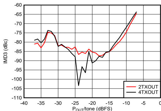
Figure 6-326. TX IMD3 vs Digital Level at 0.85 GHz
