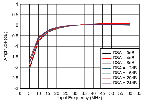
Figure 6-1. RX In-Band Gain Flatness, f_{\text{IN}} = 30\text{ MHz}
