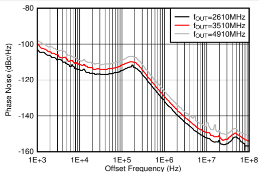
Figure 6-596. Phase Noise for 12-GHz VCO vs Offset Frequency and f_{\text{OUT}} at 25^\circ\text{C}
