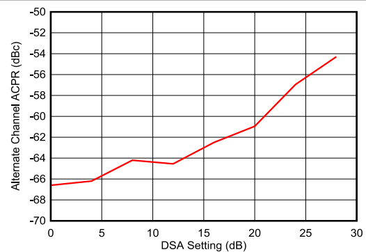
Figure 6-335. TX 20-MHz LTE alt-ACPR vs DSA at 0.85 GHz
