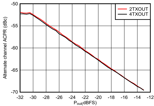
Figure 6-332. TX 20-MHz LTE alt-ACPR vs Digital Level at 0.85 GHz
