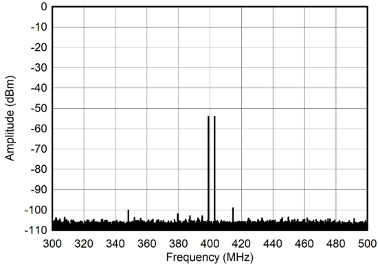
Figure 6-287. Dual Tone Spectrum at 400 MHz and -60 dBFS (±100MHz)
