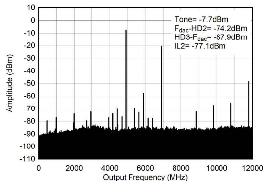
Figure 6-541. TX Single Tone (–6 dBFS) Output Spectrum at 4.9 GHz ( 0-f_{\text{DAC}} )
