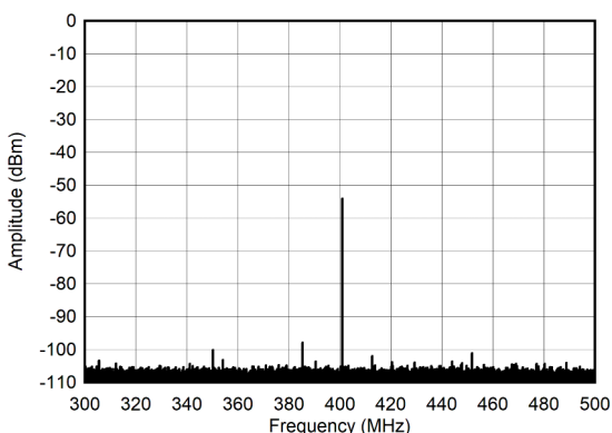
Figure 6-279. Single Tone Spectrum at 400 MHz and -60 dBFS (±100MHz)
