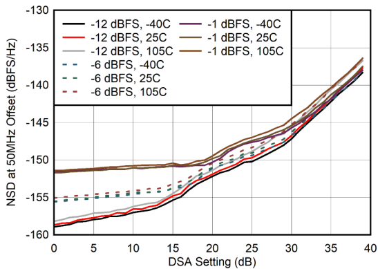
Figure 6-289. Noise Spectral Density vs DSA Setting at 400 MHz
