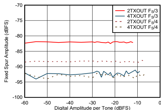
Figure 6-416. Two Tone Inband Fixed Spurs vs Digital Amplitude at 2.6 GHz
