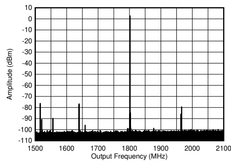
Figure 6-373. TX Single Tone (-1 dBFS) Output Spectrum at 1.8 GHz ( 0-f_{\text{DAC}} )
