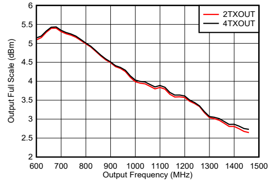
Figure 6-295. TX Full Scale vs RF Frequency and Channel at 8847.36 MSPS, Straight Mode
