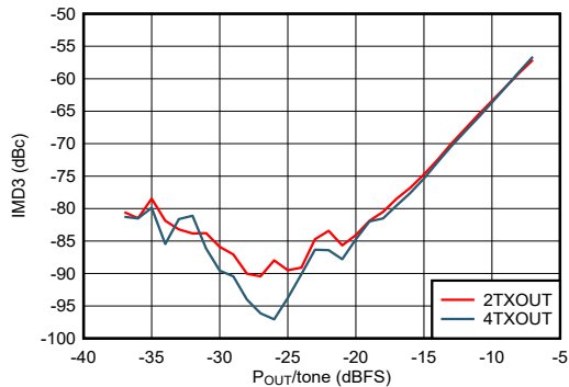
Figure 6-467. TX IMD3 vs Digital Amplitude and Dither Setting at 3.5 GHz
