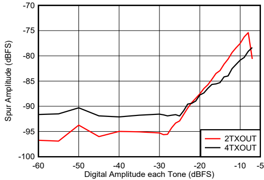
Figure 6-473. Two Tone Inband SFDR vs Digital Amplitude at 3.75 GHz
