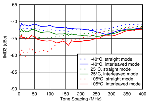
Figure 6-399. TX IMD3 vs Tone Spacing and Temperature at 2.6 GHz
