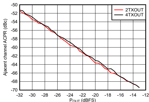
Figure 6-529. TX 20-MHz LTE ACPR vs Digital Level at 4.9 GHz
