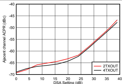
Figure 6-533. TX 20-MHz LTE ACPR vs DSA at 4.9 GHz
