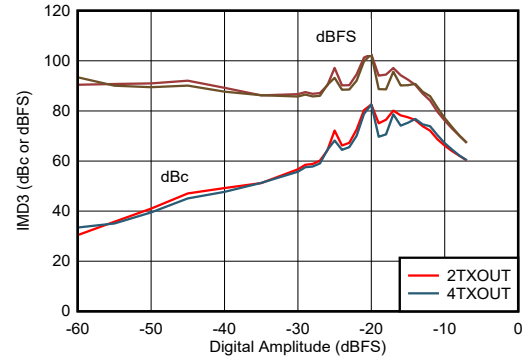
Figure 6-565. IMD3 vs Digital Amplitude and Channel at 7.1 GHz
