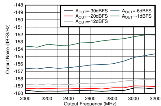
Figure 6-402. TX Single Tone Output Noise vs Frequency and Amplitude at 2.6 GHz
