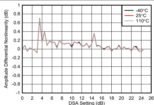
Figure 6-203. RX Uncalibrated Differential Amplitude Error at 6.851 GHz
