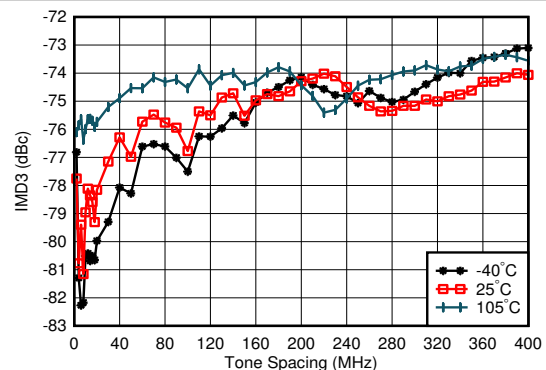
Figure 6-323. TX IMD3 vs Tone Spacing and Temperature at 0.85 GHz
