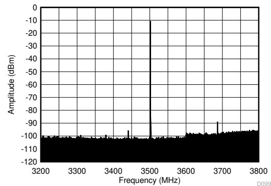
Figure 6-490. TX Single Tone (-6 dBFS) Output Spectrum at 3.5 GHz ( \pm 300 MHz)
