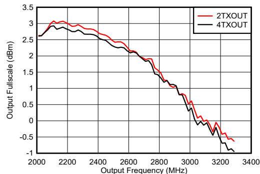
Figure 6-376. TX Full Scale vs RF Frequency at 8847.36 MSPS
