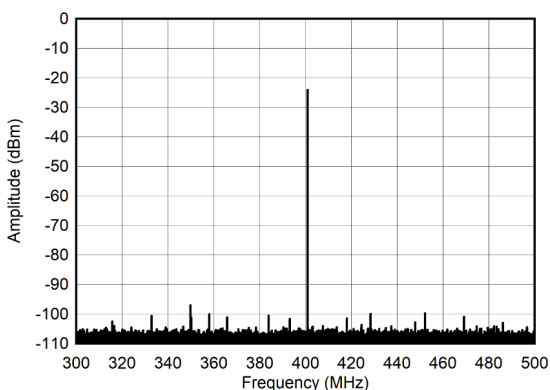
Figure 6-277. Single Tone Spectrum at 400 MHz and -30 dBFS (±100MHz)
