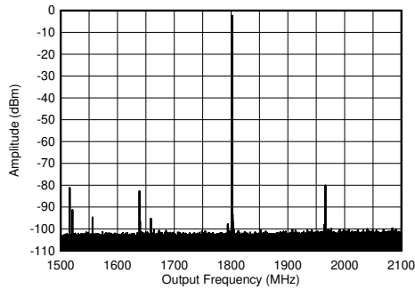
Figure 6-372. TX Single Tone (-6 dBFS) Output Spectrum at 1.8 GHz (±300 MHz)
