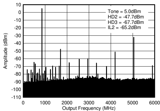
Figure 6-344. TX Single Tone (-6 dBFS) Output Spectrum at 0.85 GHz ( 0-f_{\text{DAC}} )
