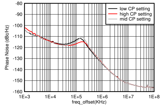
Figure 6-599. Phase Noise for 12-GHz VCO vs Offset Frequency and CP Setting at f_{OUT} = 2.6 GHz
