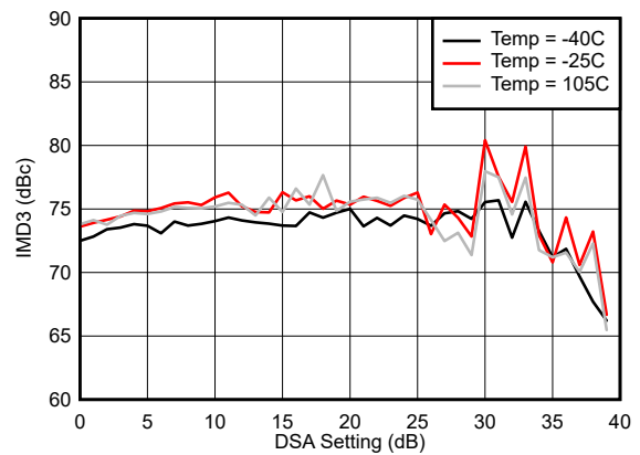
Figure 6-569. IMD3 vs DSA Setting and Temperature at 7.1 GHz
