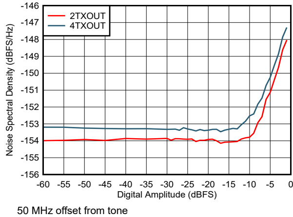
Figure 6-576. NSD vs Digital Amplitude and Channel at 7.1 GHz
