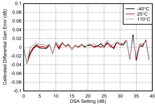
Figure 6-552. Calibrated Differential Gain Error vs Temperature at 7.1 GHz
