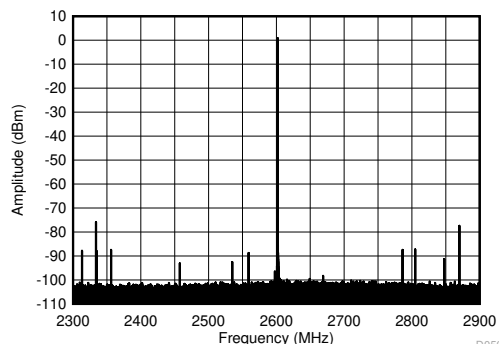
Figure 6-428. TX Single Tone (-1 dBFS) Output Spectrum at 2.6 GHz ( \pm 300 MHz)
