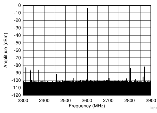
Figure 6-418. TX Single Tone (-12 dBFS) Output Spectrum at 2.6 GHz ( \pm 300 MHz)
