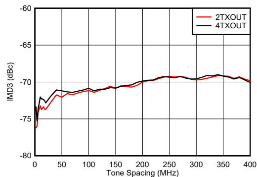
Figure 6-398. TX IMD3 vs Tone Spacing and Channel at 2.6 GHz
