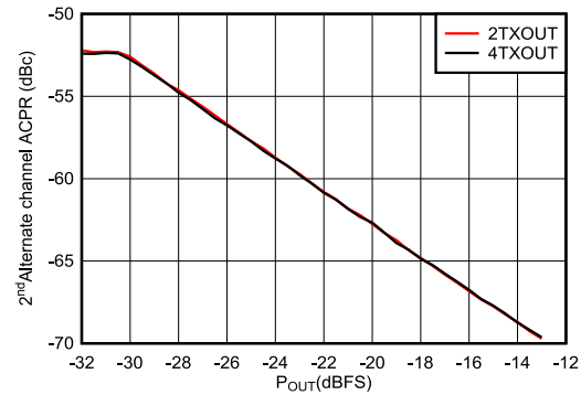
Figure 6-333. TX 20-MHz LTE alt2-ACPR vs Digital Level at 0.85 GHz
