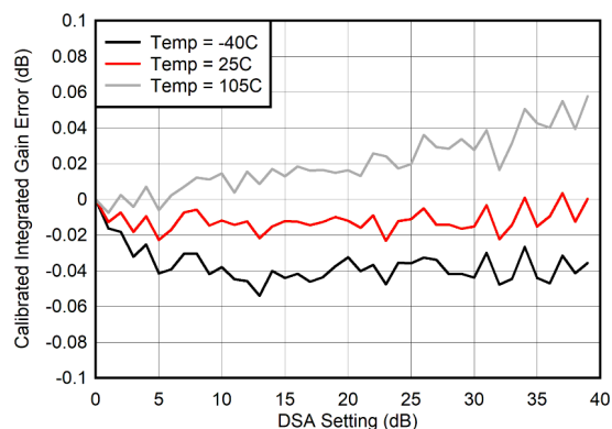
Figure 6-265. Calibrated TX Integrated Gain Error (INL) at 400 MHz
