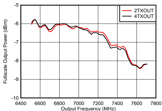
Figure 6-546. TX Full Scale vs RF Frequency and Channel
