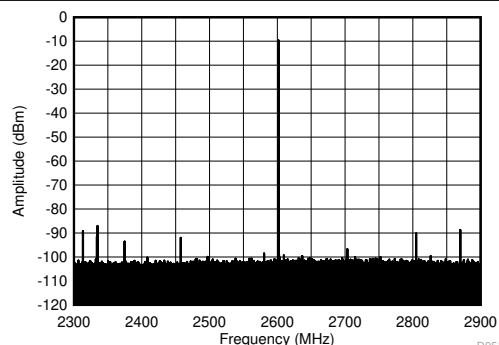
Figure 6-416. Two Tone Inband Fixed Spurs vs Digital Amplitude at 2.6 GHz
