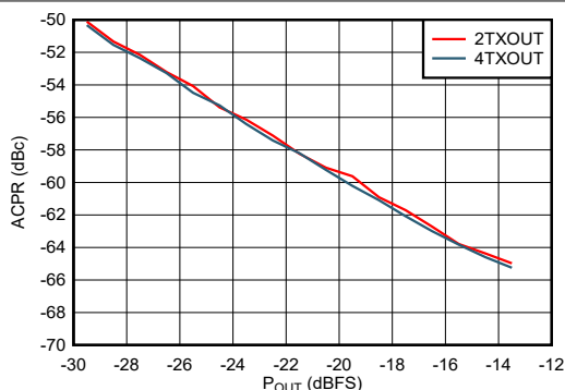
Figure 6-405. TX 20-MHz LTE alt-ACPR vs Digital Level at 2.6 GHz
