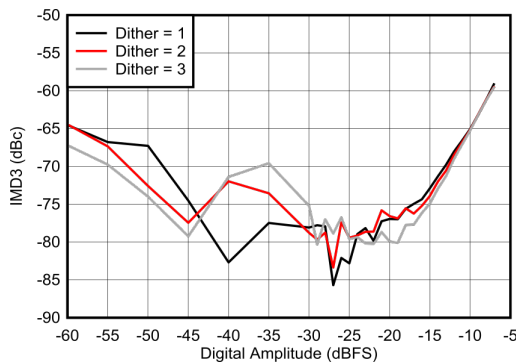
Figure 6-441. IMD3 vs Digital Amplitude and Dither at 2.6 GHz
