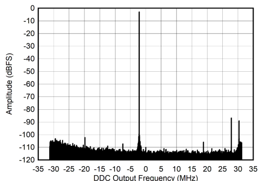
Figure 6-13. RX Output FFT at 5 MHz
