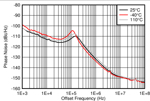
Figure 6-623. Phase Noise for 8-GHz VCO vs Offset Frequency and Temperature at f_{OUT} = 1910 MHz
