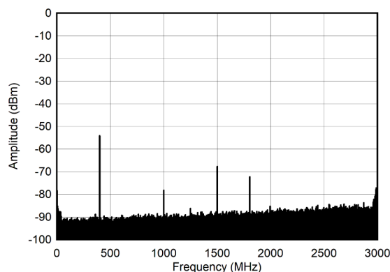
Figure 6-278. Single Tone Spectrum at 400 MHz and -60 dBFS (Nyquist)
