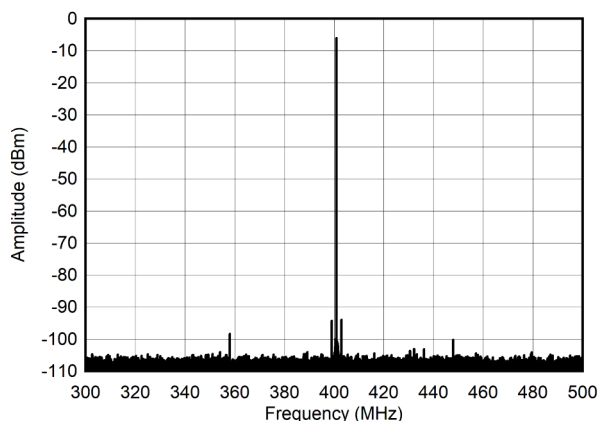
Figure 6-275. Single Tone Spectrum at 400 MHz and -12 dBFS (±100MHz)
