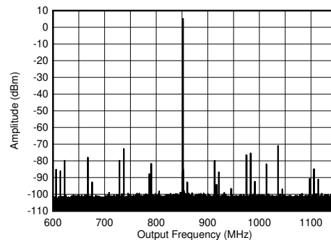
Figure 6-345. TX Single Tone (-6 dBFS) Output Spectrum at 0.85 GHz ( \pm 300 MHz)
