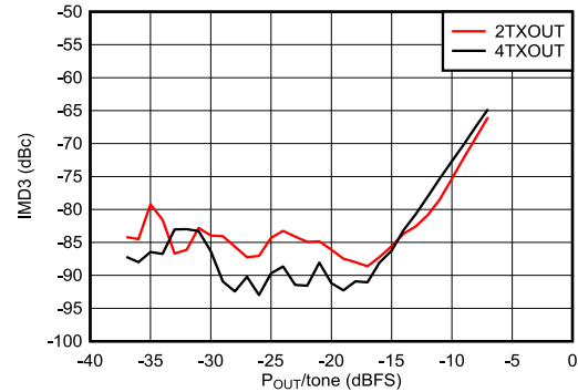
Figure 6-327. TX IMD3 vs Digital Level at 0.85 GHz
