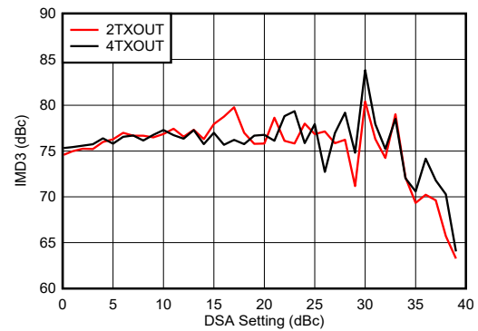
Figure 6-567. IMD3 vs DSA Setting and Channel at 7.1 GHz
