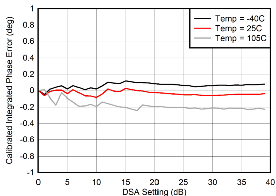
Figure 6-269. Calibrated TX Integrated Phase Error (INL) at 400 MHz
