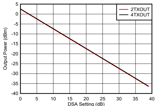
Figure 6-379. TX Output Power vs DSA Setting and Channel at 2.6 GHz
