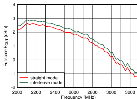
Figure 6-376. TX Full Scale vs RF Frequency at 8847.36 MSPS
