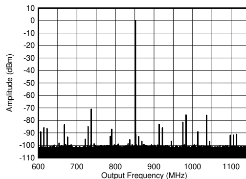
Figure 6-351. TX Single Tone (-6 dBFS) Output Spectrum at 0.85 GHz ( \pm 300 MHz)
