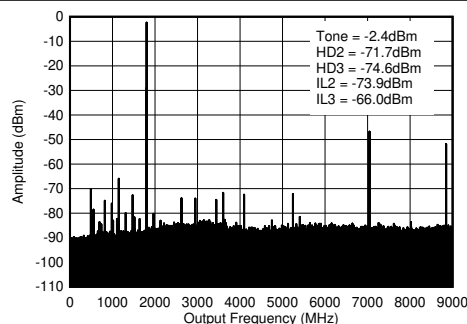
Figure 6-369. TX Single Tone (-12 dBFS) Output Spectrum at 1.8 GHz ( 0-f_{\text{DAC}} )
