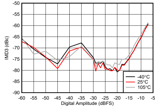
Figure 6-440. IMD3 vs Digital Amplitude and Temperature at 2.6 GHz
