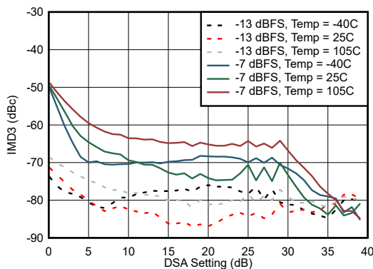
Figure 6-257. IMD3 vs DSA Setting at 30 MHz
