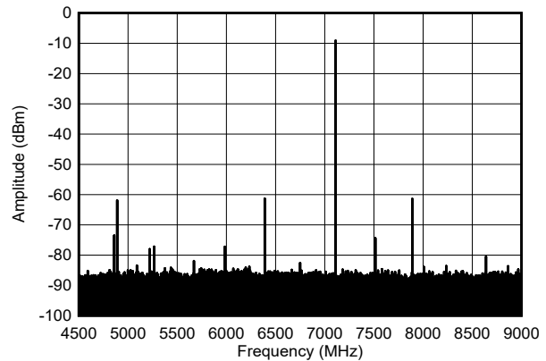
Figure 6-579. Single Tone Output Spectrum at 7.1 GHz, -1 dBFS (Nyquist)
