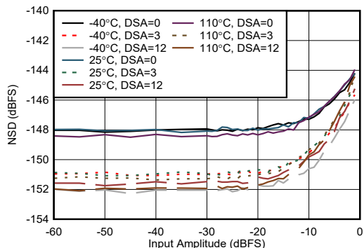
Figure 6-216. RX NSD vs Input Amplitude at 6.851 GHz
