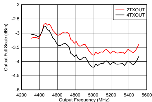
Figure 6-501. TX Full Scale vs RF Frequency and Channel at 5898.24 MSPS, Mixed Mode, 2nd Nyquist Zone
