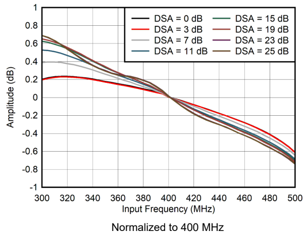
Figure 6-29. RX In-Band Gain Flatness, f_{\text{IN}} = 400 MHz
