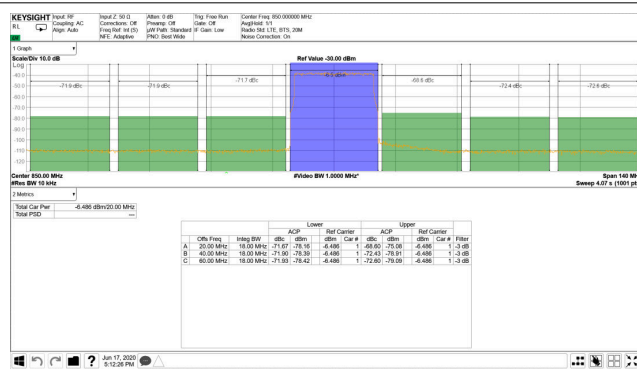
Figure 6-330. TX 20-MHz LTE Output Spectrum at 0.85 GHz
