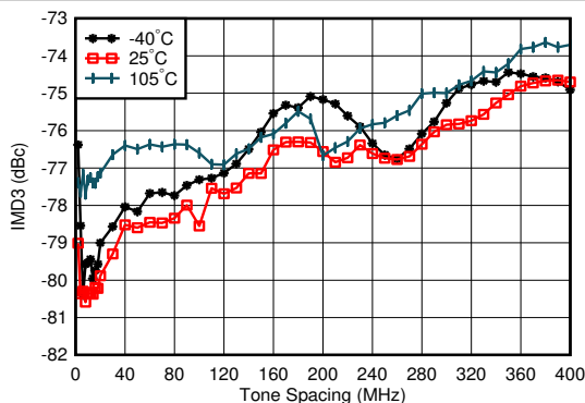
Figure 6-322. TX IMD3 vs Tone Spacing and Channel at 0.85 GHz
