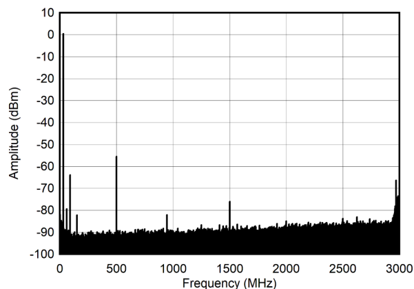
Figure 6-242. Single Tone Spectrum at 30 MHz and -6 dBFS (Nyquist)
