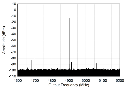
Figure 6-544. TX Single Tone (–12 dBFS) Output Spectrum at 4.9 GHz (±300 MHz)
