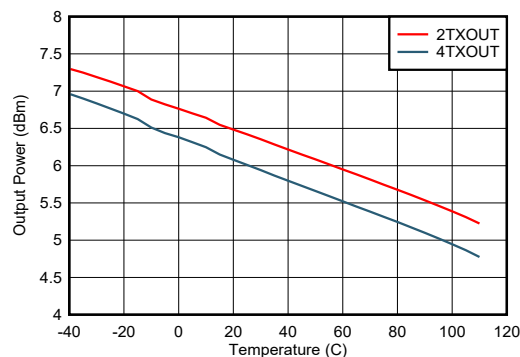
Figure 6-260. TX Output Fullscale vs Temperature at 400 MHz
