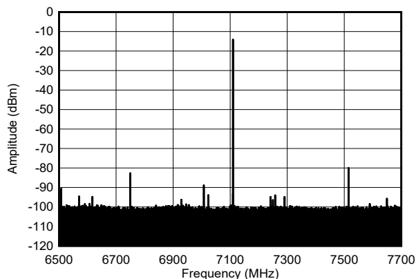
Figure 6-582. Single Tone Output Spectrum at 7.1 GHz, -6 dBFS (narrow span)
