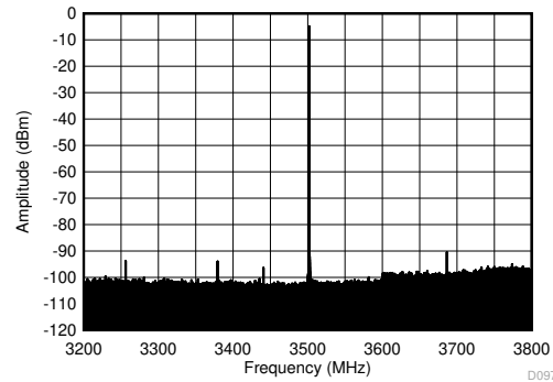
Figure 6-490. TX Single Tone (-6 dBFS) Output Spectrum at 3.5 GHz ( \pm 300 MHz)
