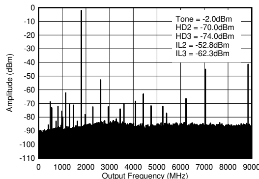
f_{\text{DAC}} = 8847.36\text{ MSPS} , interleave mode, 1.8 GHz matching, includes PCB and cable losses. \text{ILn} = f_s/n \pm f_{\text{OUT}} . Figure 6-365. TX Single Tone (-6 dBFS) Output Spectrum at 1.8 GHz ( 0-f_{\text{DAC}} )
