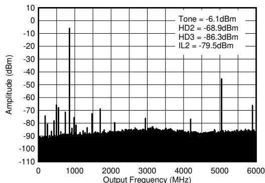
Figure 6-346. TX Single Tone (-1 dBFS) Output Spectrum at 0.85 GHz ( 0-f_{\text{DAC}} )
