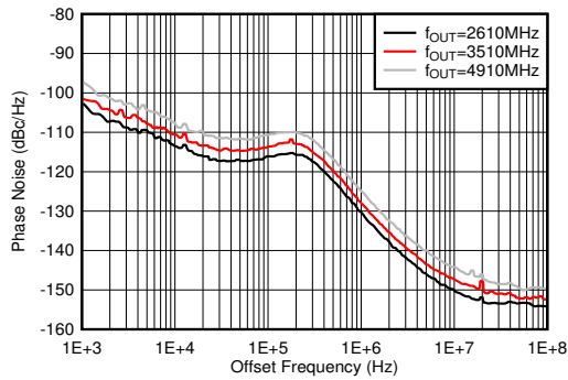
Figure 6-610. Phase Noise for 10-GHz VCO vs Offset Frequency and f_{OUT} at 110°C
