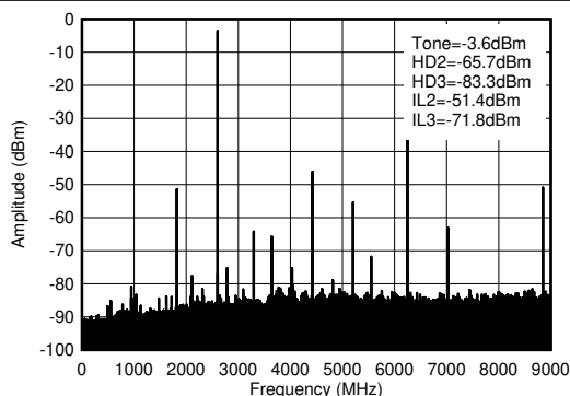
Figure 6-417. TX Single Tone (-12 dBFS) Output Spectrum at 2.6 GHz ( 0-f_{\text{DAC}} )
