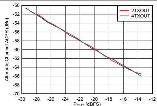
Figure 6-406. TX 20-MHz LTE alt2-ACPR vs Digital Level at 2.6 GHz
