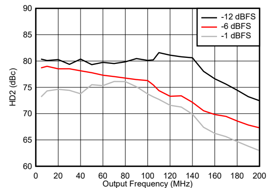
Figure 6-258. HD2 vs Frequency 0 - 200 MHz
