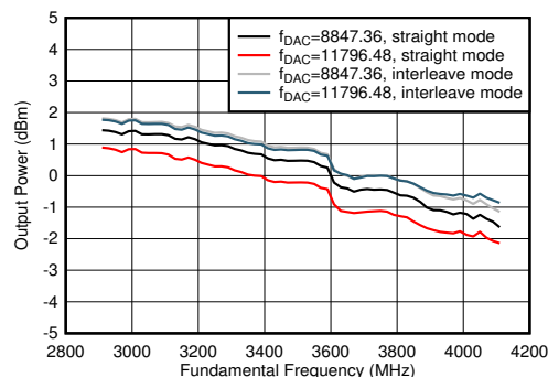
Figure 6-446. TX Output Power vs Frequency
