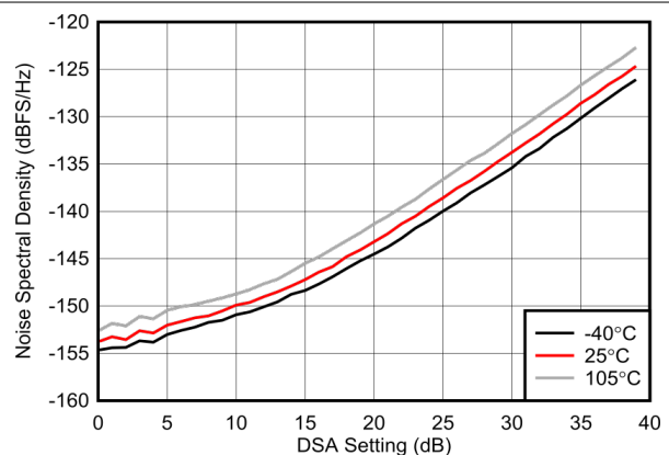
Figure 6-575. NSD vs DSA Setting and Temperature at 7.1 GHz
