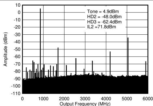
Figure 6-350. TX Single Tone (-6 dBFS) Output Spectrum at 0.85 GHz ( 0-f_{\text{DAC}} )
