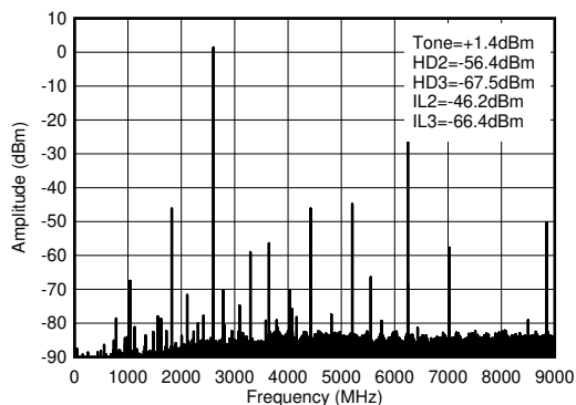
Figure 6-421. TX Single Tone (-1 dBFS) Output Spectrum at 2.6 GHz ( 0-f_{\text{DAC}} )
