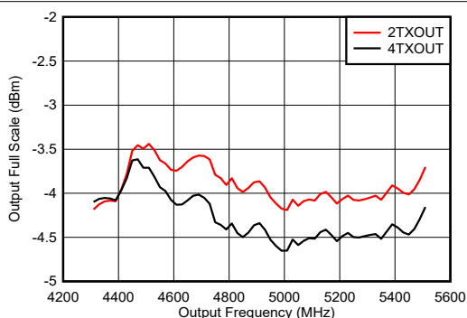
Figure 6-500. TX Full Scale vs RF Frequency and Channel at 11796.48 MSPS
