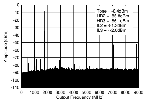
Figure 6-367. TX Single Tone (-1 dBFS) Output Spectrum at 1.8 GHz ( 0-f_{\text{DAC}} )
