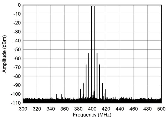
Figure 6-281. Dual Tone Spectrum at 400 MHz and -7 dBFS (±100MHz)
