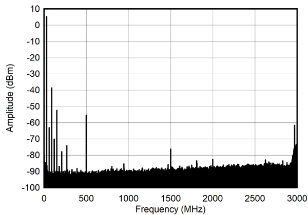
Figure 6-240. Single Tone Spectrum at 30 MHz and -1 dBFS (Nyquist)
