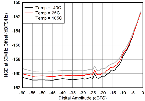
Figure 6-288. Noise Spectral Density vs Digital Amplitude at 400 MHz
