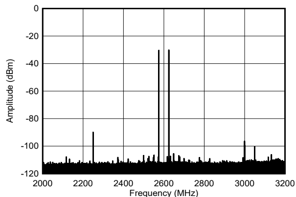
Figure 6-434. TX Dual Tone Output Spectrum at 2.6 GHz, -30dBFS each ( \pm 600 MHz)
