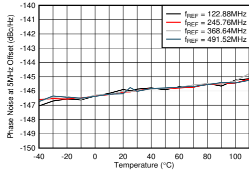
Figure 6-605. Phase Noise for 12-GHz VCO at 5-MHz Offset vs Temperature and f_{REF} at f_{OUT} = 2.6 GHz
