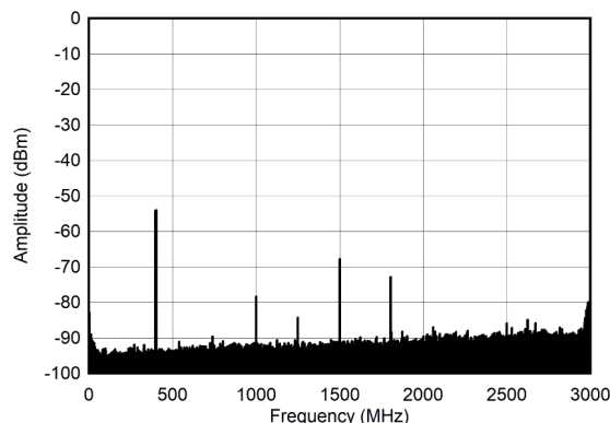
Figure 6-286. Dual Tone Spectrum at 400 MHz and -60 dBFS (Nyquist)
