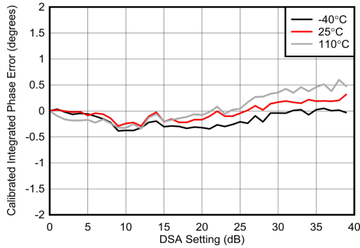
Figure 6-564. Calibrated Integrated Phase Error vs Temperature at 7.1 GHz
