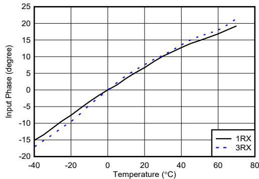
Figure 6-83. RX Input Phase vs Temperature and DSA at f_{\text{IN}} = 1.75 \text{ GHz}
