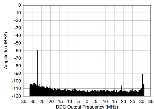
Figure 6-14. RX Output FFT at 5 MHz
