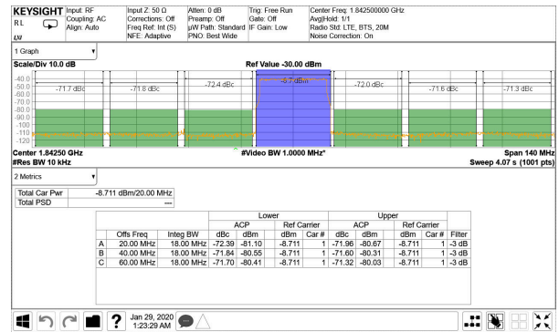
Figure 6-355. TX 20-MHz LTE Output Spectrum at 1.8425 GHz
