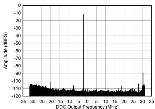
Figure 6-15. RX Output FFT at 30 MHz
