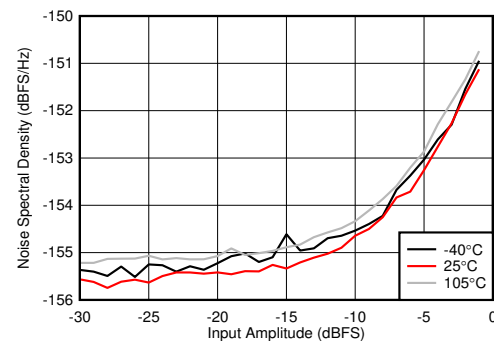
Figure 6-116. RX Noise Spectral Density vs Input Amplitude and Temperature at 2.6 GHz
