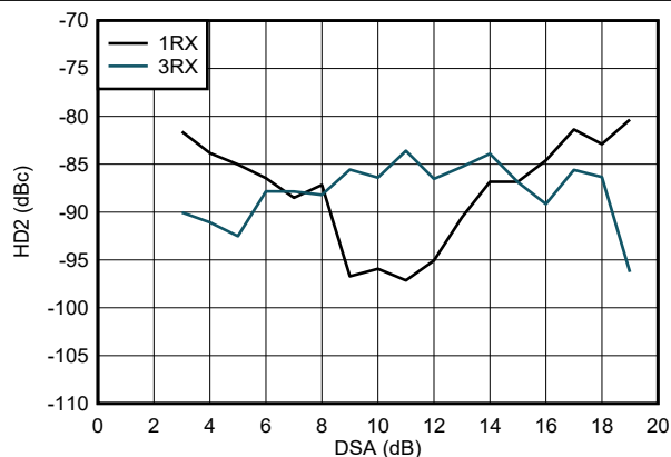
Figure 6-99. RX HD2 vs DSA Setting and Channel at 1.9 GHz
