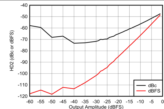
Figure 6-292. HD2 vs Amplitude at 400 MHz
