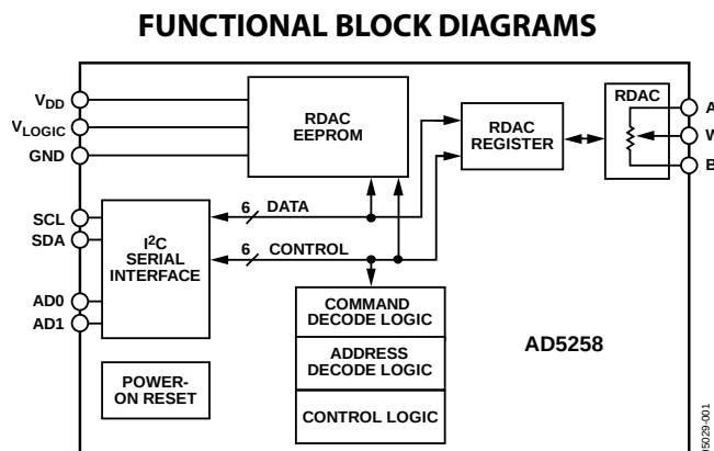
Figure 1. Block Diagram
