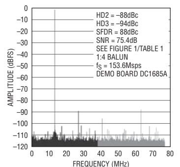
LTC6417 Driving LTC2209 16-Bit ADC 32K Point FFT, f_{\text{IN}} = 140\text{MHz} , -1\text{dBFS} , \text{PGA} = 0
