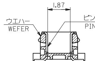
SECT. Z-Z
