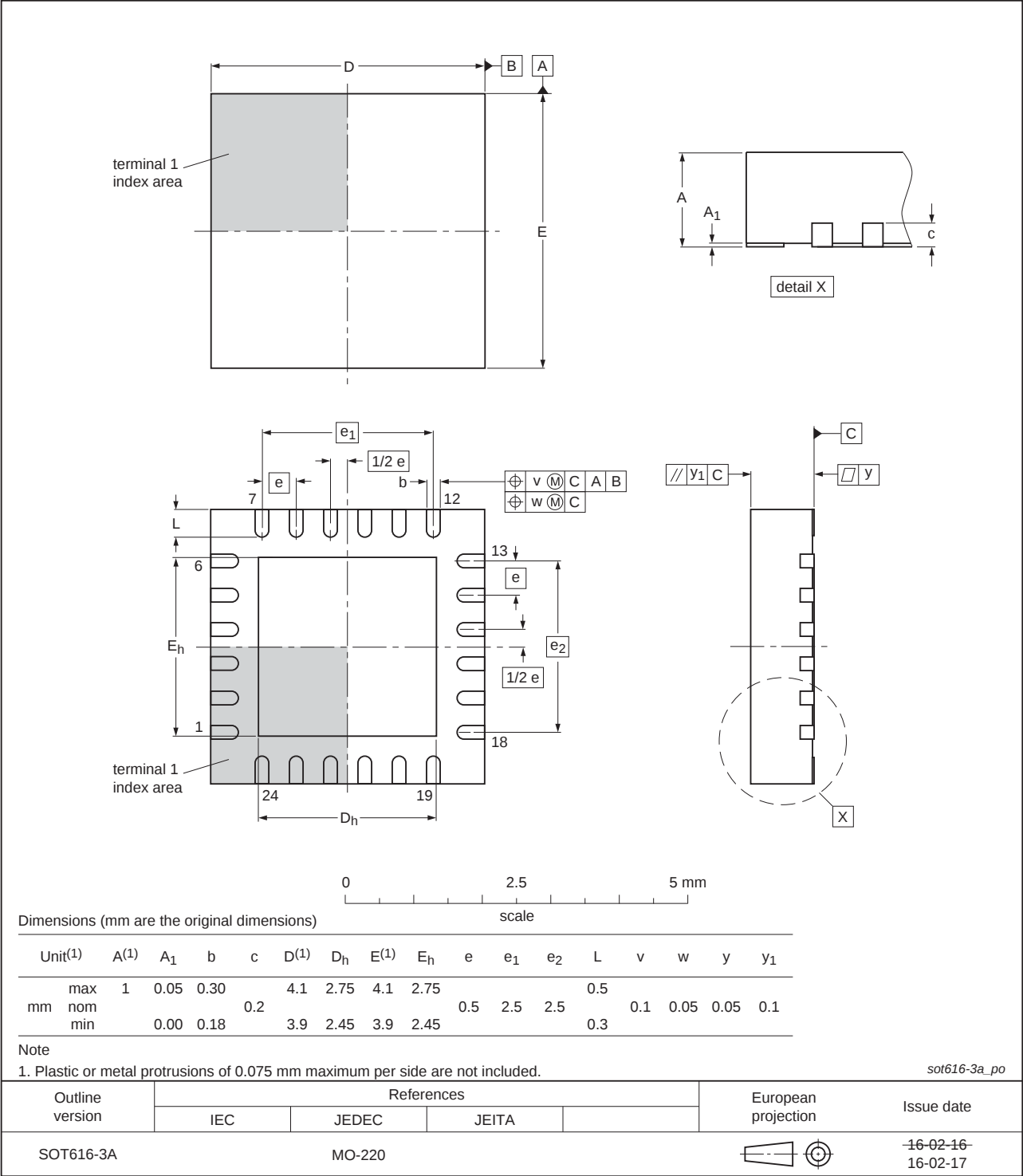
Fig 19. Package outline SOT616-3 (HVQFN24)
