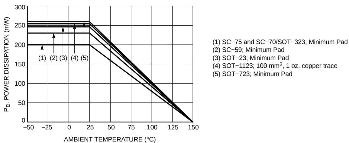
Figure 1. Derating Curve
