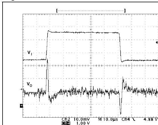
Figure 19. Line transient
