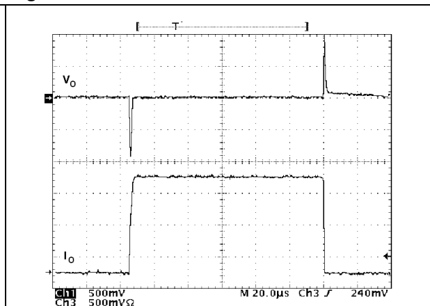
Figure 20. Load transient
