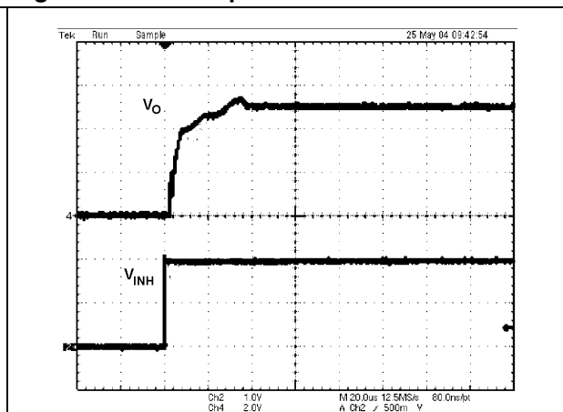
Figure 22. Start-up time 1.5A
