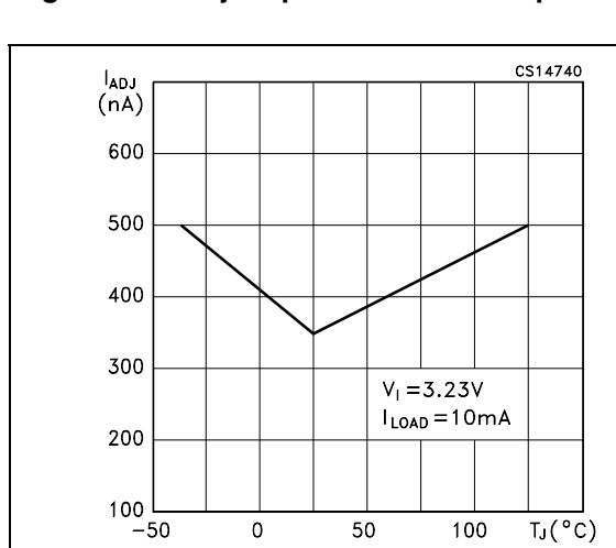
Figure 15. Adjust pin current vs temperature
