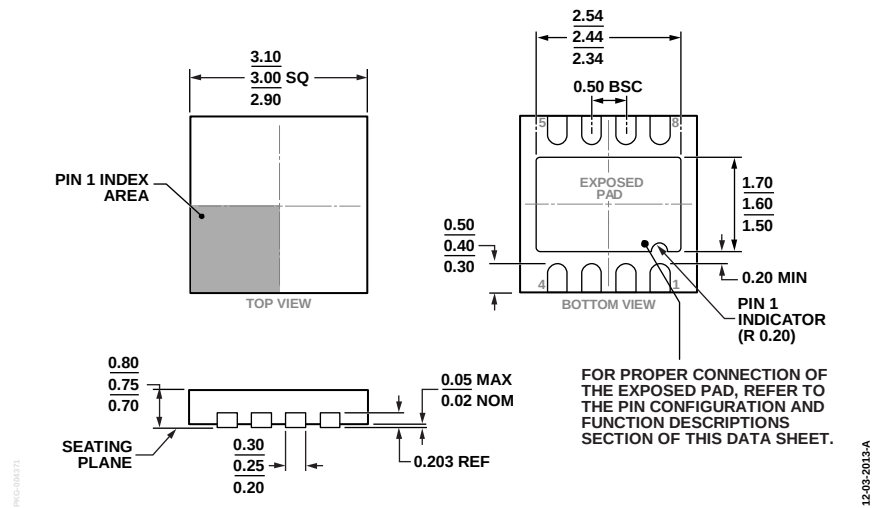
Figure 65. 8-Lead Lead Frame Chip Scale Package [LFCSP_WD] 3 mm × 3 mm Body, Very Very Thin, Dual Lead (CP-8-21)
