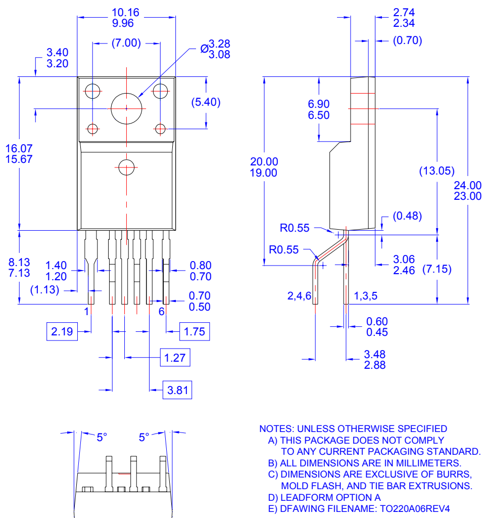
Figure 26. TO-220F-6L (W-Forming)
