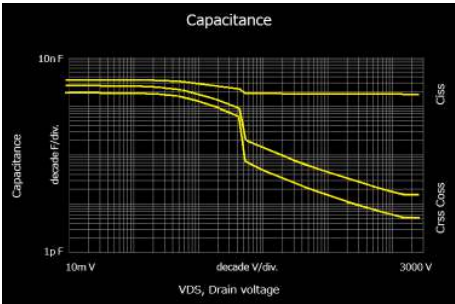
Ciss/Coss/Crss measurement up to 3kV
