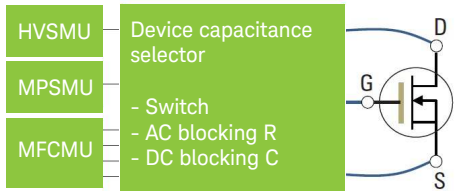
Device capacitance selector for automated CV measurement
