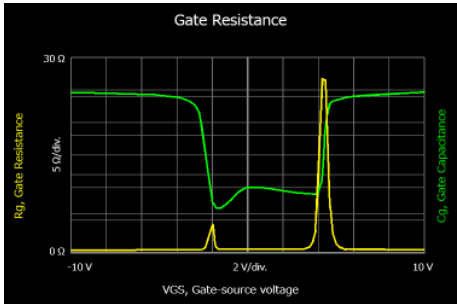
Gate Resistance Measurement
