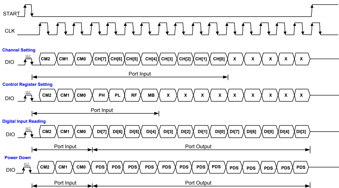
Figure-3 Timing Diagram of Whole Commands
