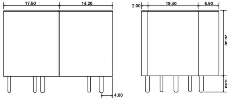
S = Sealed
