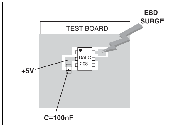
Figure 9. ESD behavior: measurement conditions (with coupling capacitance)
