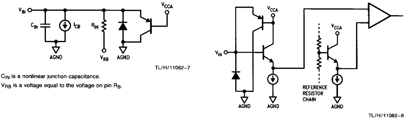
FIGURE 2. Simplified Analog Input Circuits
