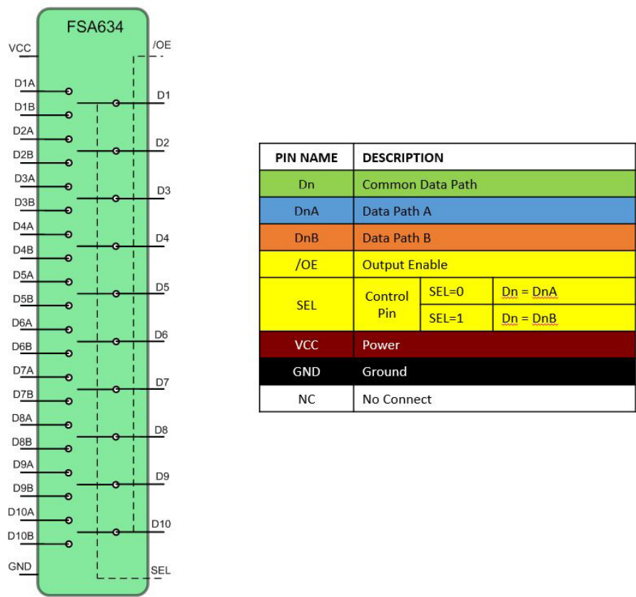
Figure 2. Analog Symbol
