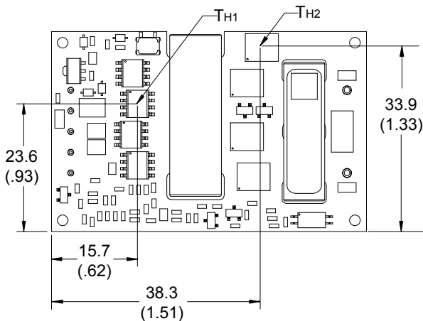
Figure 13. Locations of the thermal reference temperature measurement points T_{H1} and T_{H2} .
