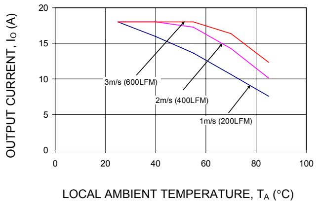
Figure 15. Output Current Derating for the QBW018A0B-TZ in the Transverse Orientation with baseplate; Airflow Direction From Vin(-) to Vin(+); Vin = 48V.
