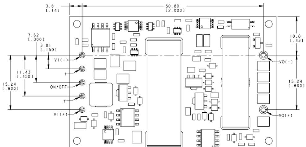
BOTTOM VIEW
