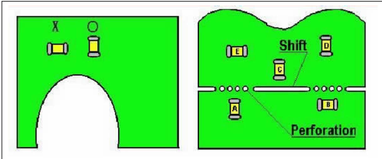
Figure 3 Component Layout
