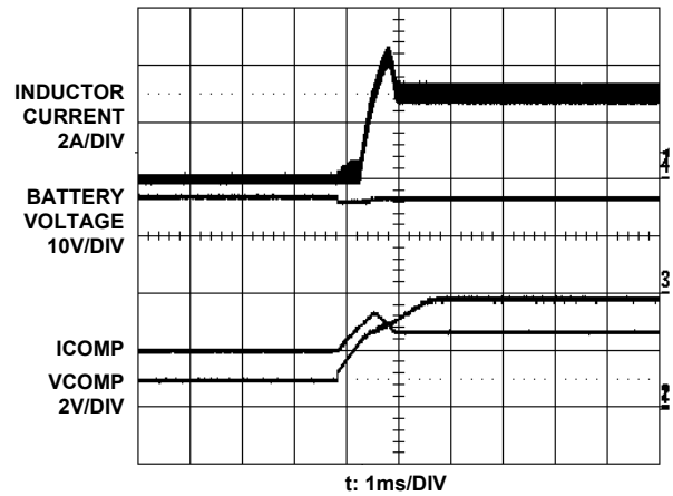
FIGURE 10. BATTERY INSERTION
