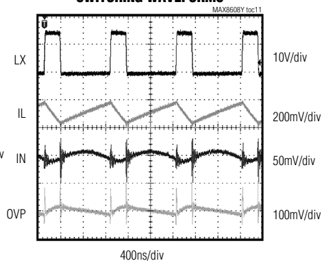
SWITCHING WAVEFORMS
